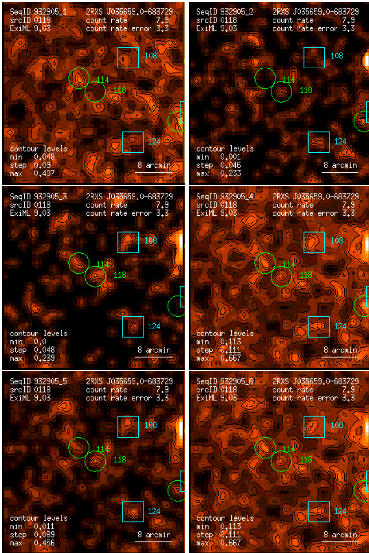
Figure 118: RASS 932905: detection 0118: band rate images, Gaussian filter: (1) PSPC channels 11 – 41, (2) 52 – 90, (3) 91 – 201, (4) 11 – 235, (5) 52 – 201, (6) 11 – 201. Broad band rates in counts/ks. Band rate contour levels in counts/ks/arcmin 2 .
