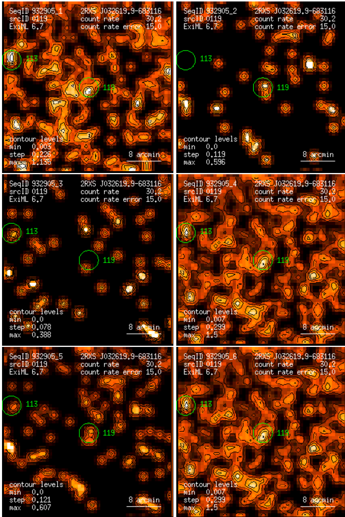
Figure 119: RASS 932905: detection 0119: band rate images, Gaussian filter: (1) PSPC channels 11 – 41, (2) 52 – 90, (3) 91 – 201, (4) 11 – 235, (5) 52 – 201, (6) 11 – 201. Broad band rates in counts/ks. Band rate contour levels in counts/ks/arcmin 2 .
