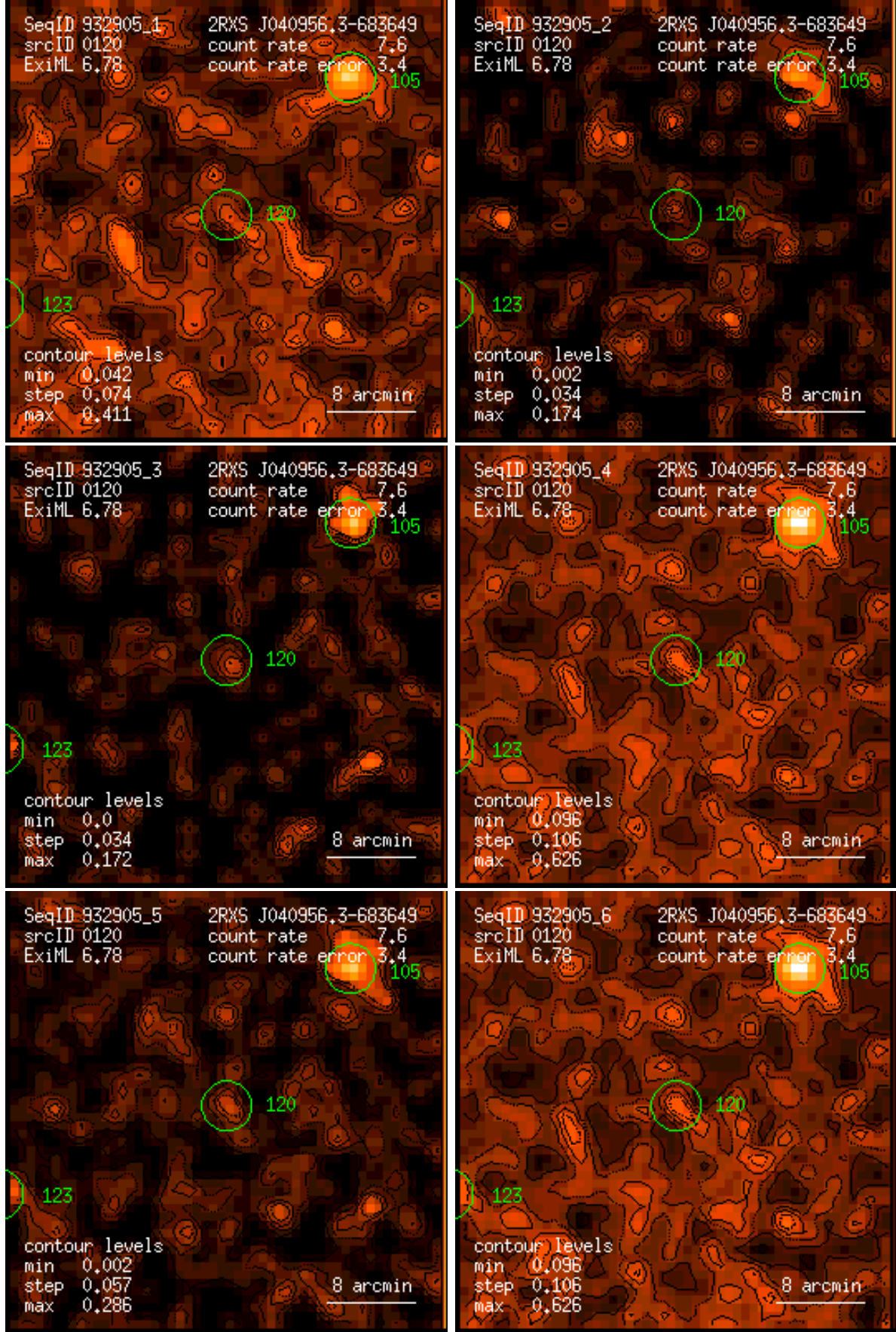
Figure 120: RASS 932905: detection 0120: band rate images, Gaussian filter: (1) PSPC channels 11 – 41, (2) 52 – 90, (3) 91 – 201, (4) 11 – 235, (5) 52 – 201, (6) 11 – 201. Broad band rates in counts/ks. Band rate contour levels in counts/ks/arcmin 2 .
