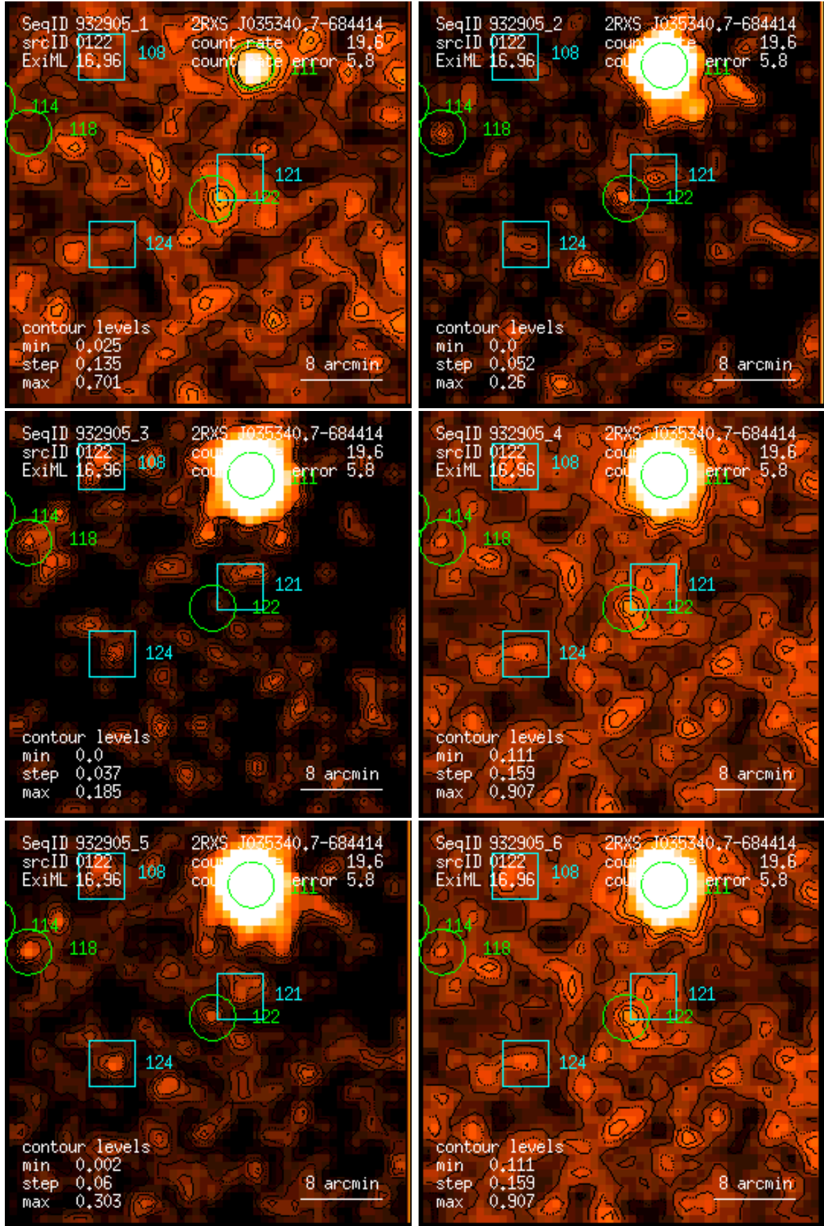
Figure 122: RASS 932905: detection 0122: band rate images, Gaussian filter: (1) PSPC channels 11 – 41, (2) 52 – 90, (3) 91 – 201, (4) 11 – 235, (5) 52 – 201, (6) 11 – 201. Broad band rates in counts/ks. Band rate contour levels in counts/ks/arcmin 2 .
