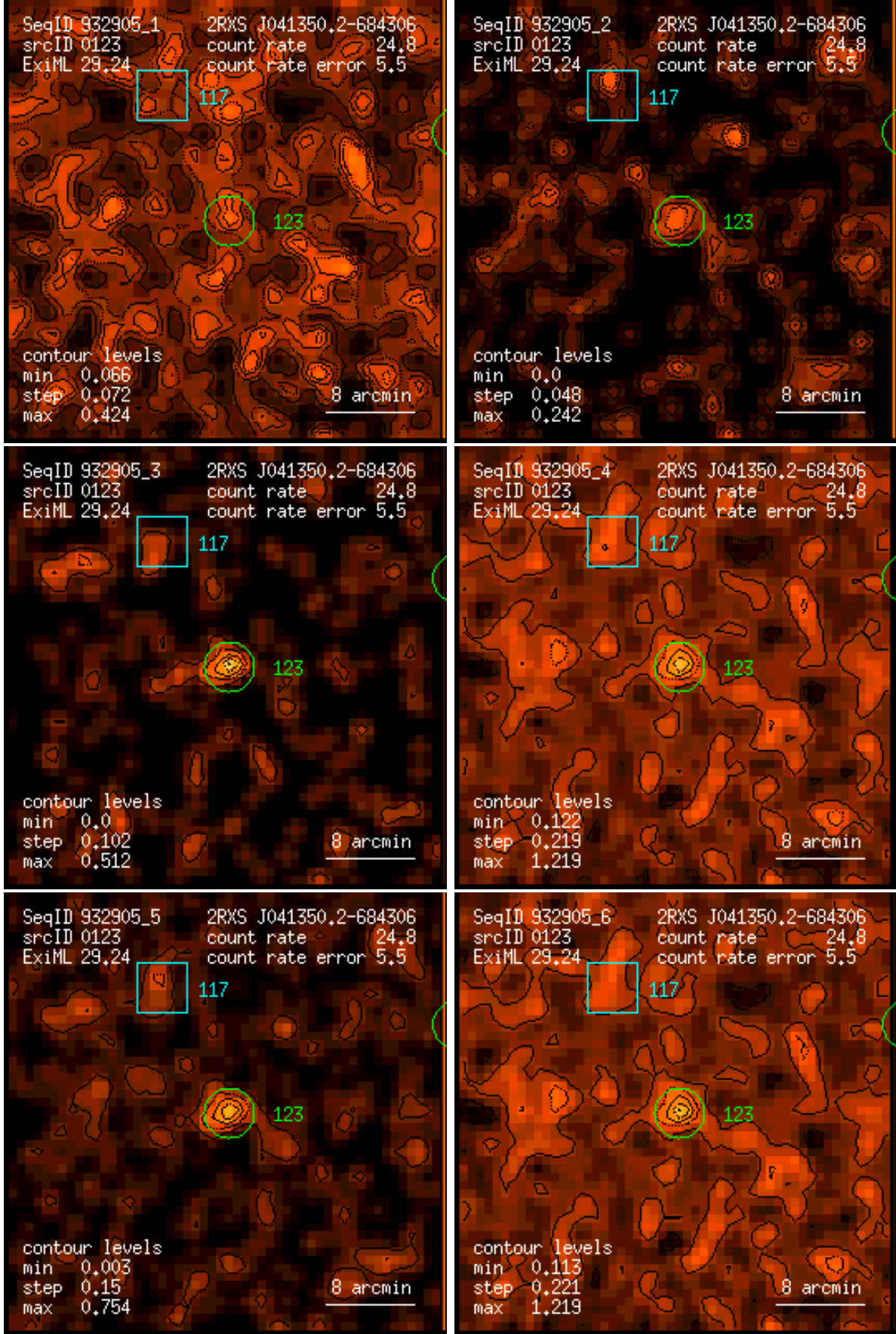
Figure 123: RASS 932905: detection 0123: band rate images, Gaussian filter: (1) PSPC channels 11 – 41, (2) 52 – 90, (3) 91 – 201, (4) 11 – 235, (5) 52 – 201, (6) 11 – 201. Broad band rates in counts/ks. Band rate contour levels in counts/ks/arcmin 2 .
