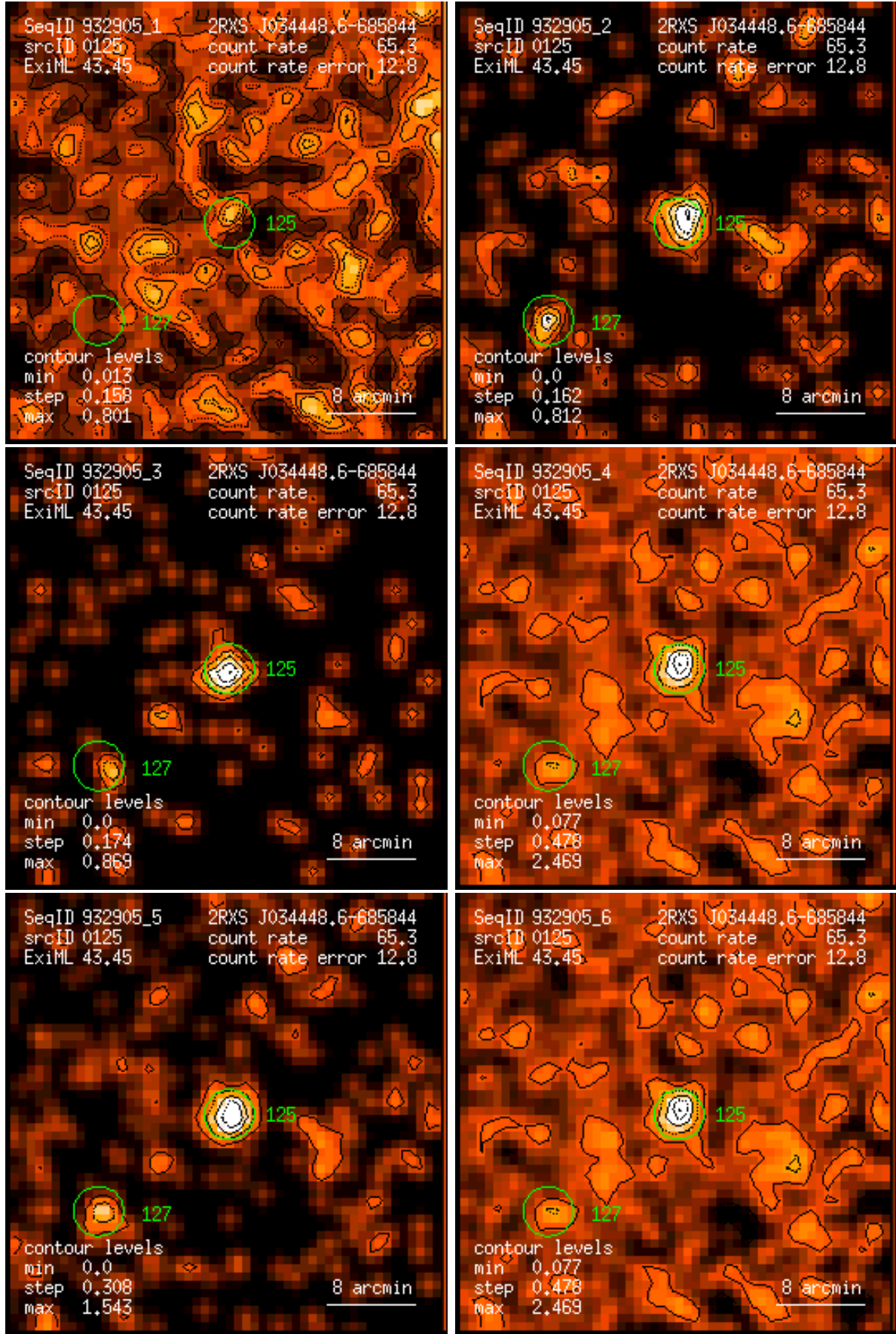
Figure 125: RASS 932905: detection 0125: band rate images, Gaussian filter: (1) PSPC channels 11 – 41, (2) 52 – 90, (3) 91 – 201, (4) 11 – 235, (5) 52 – 201, (6) 11 – 201. Broad band rates in counts/ks. Band rate contour levels in counts/ks/arcmin 2 .
