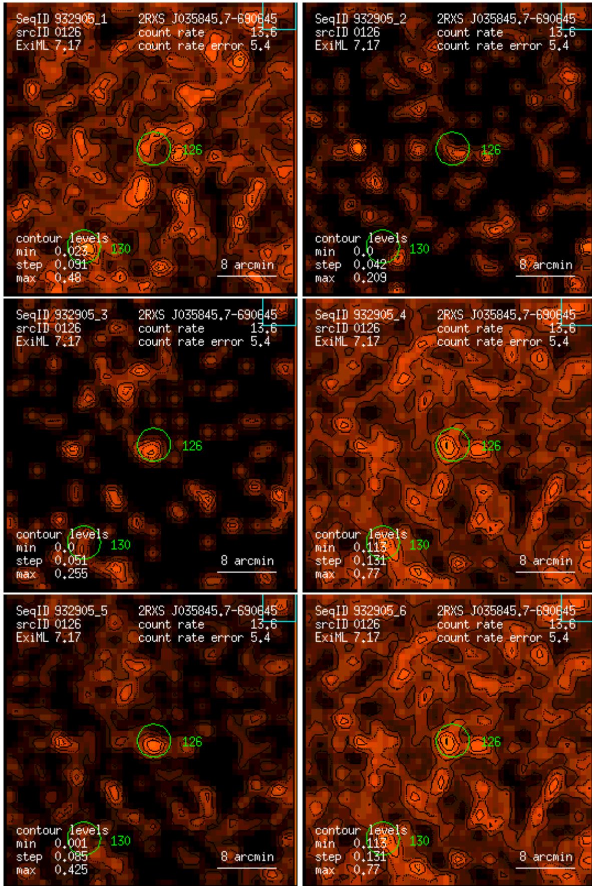
Figure 126: RASS 932905: detection 0126: band rate images, Gaussian filter: (1) PSPC channels 11 – 41, (2) 52 – 90, (3) 91 – 201, (4) 11 – 235, (5) 52 – 201, (6) 11 – 201. Broad band rates in counts/ks. Band rate contour levels in counts/ks/arcmin 2 .
