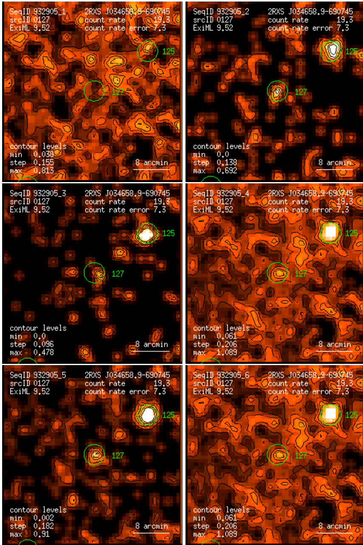
Figure 127: RASS 932905: detection 0127: band rate images, Gaussian filter: (1) PSPC channels 11 – 41, (2) 52 – 90, (3) 91 – 201, (4) 11 – 235, (5) 52 – 201, (6) 11 – 201. Broad band rates in counts/ks. Band rate contour levels in counts/ks/arcmin 2 .
