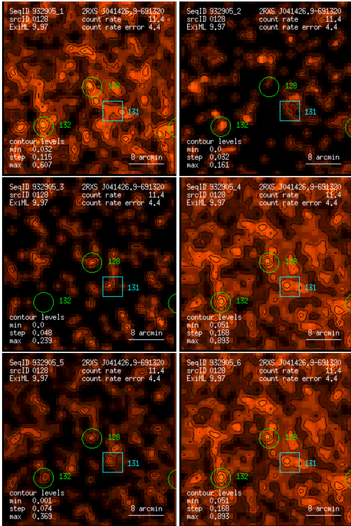
Figure 128: RASS 932905: detection 0128: band rate images, Gaussian filter: (1) PSPC channels 11 – 41, (2) 52 – 90, (3) 91 – 201, (4) 11 – 235, (5) 52 – 201, (6) 11 – 201. Broad band rates in counts/ks. Band rate contour levels in counts/ks/arcmin 2 .
