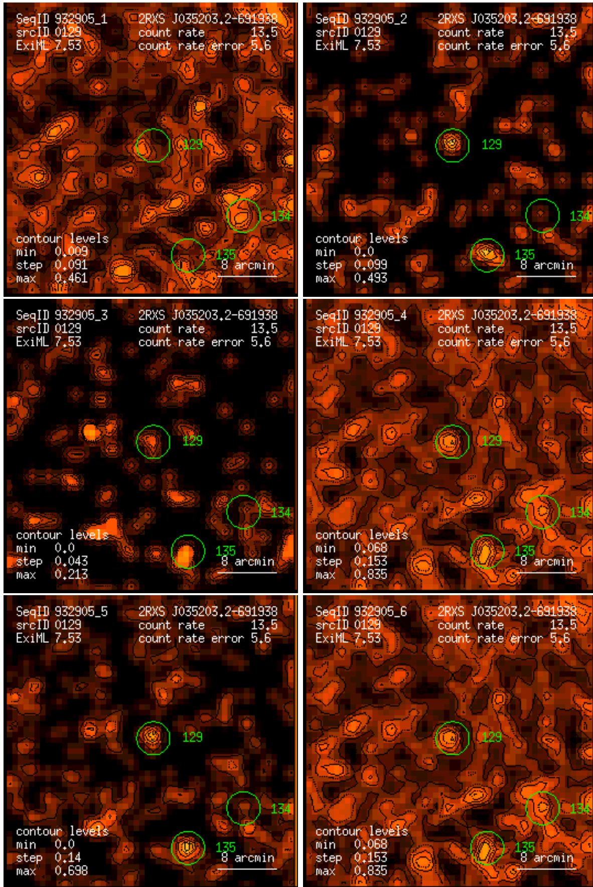
Figure 129: RASS 932905: detection 0129: band rate images, Gaussian filter: (1) PSPC channels 11 – 41, (2) 52 – 90, (3) 91 – 201, (4) 11 – 235, (5) 52 – 201, (6) 11 – 201. Broad band rates in counts/ks. Band rate contour levels in counts/ks/arcmin 2 .
