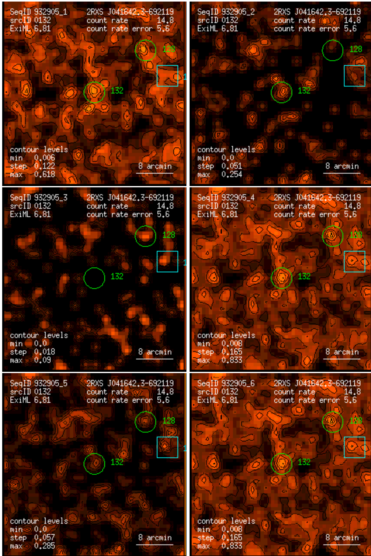
Figure 132: RASS 932905: detection 0132: band rate images, Gaussian filter: (1) PSPC channels 11 – 41, (2) 52 – 90, (3) 91 – 201, (4) 11 – 235, (5) 52 – 201, (6) 11 – 201. Broad band rates in counts/ks. Band rate contour levels in counts/ks/arcmin 2 .
