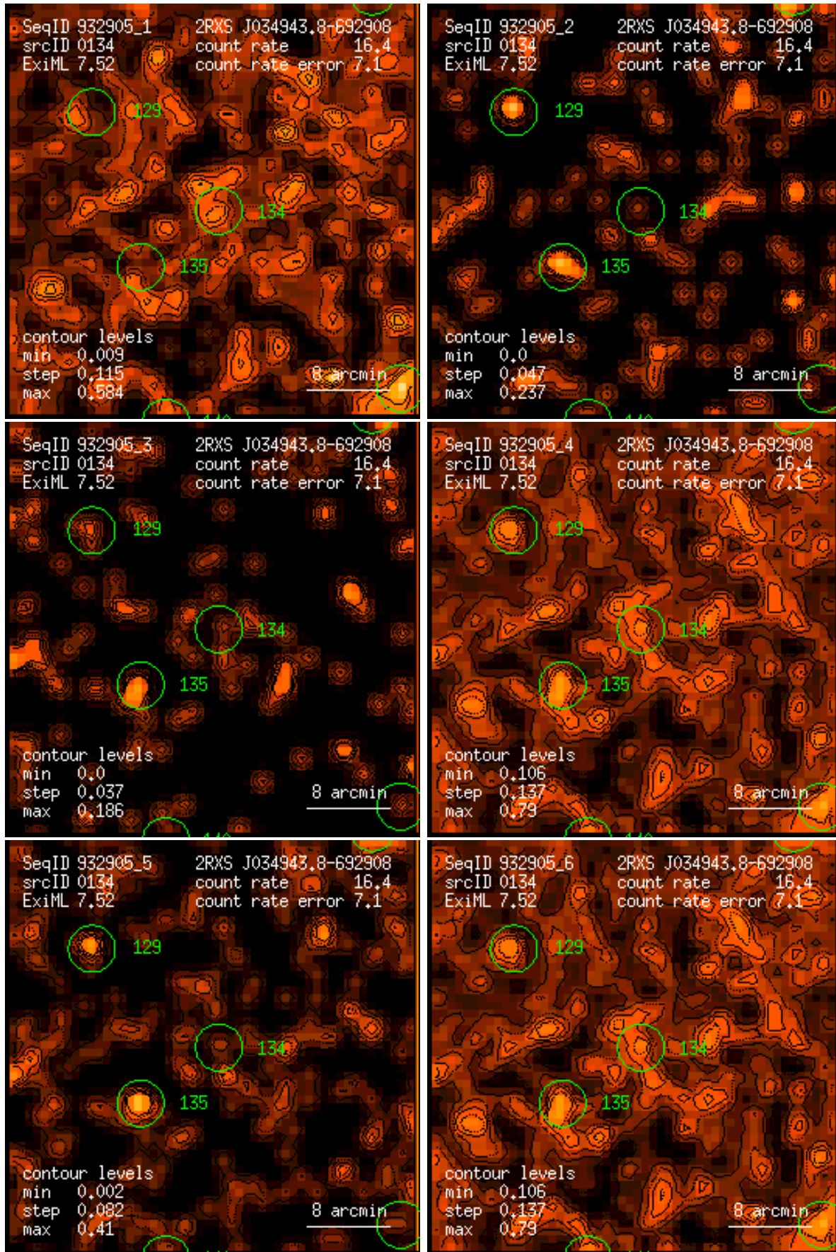
Figure 134: RASS 932905: detection 0134: band rate images, Gaussian filter: (1) PSPC channels 11 – 41, (2) 52 – 90, (3) 91 – 201, (4) 11 – 235, (5) 52 – 201, (6) 11 – 201. Broad band rates in counts/ks. Band rate contour levels in counts/ks/arcmin 2 .
