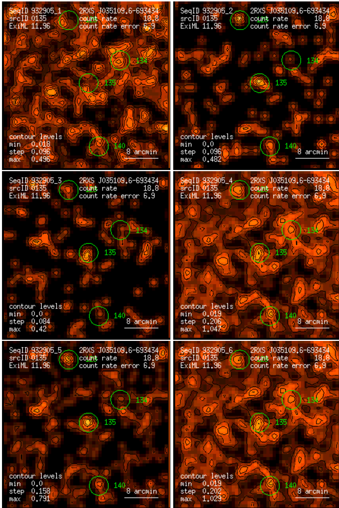
Figure 135: RASS 932905: detection 0135: band rate images, Gaussian filter: (1) PSPC channels 11 – 41, (2) 52 – 90, (3) 91 – 201, (4) 11 – 235, (5) 52 – 201, (6) 11 – 201. Broad band rates in counts/ks. Band rate contour levels in counts/ks/arcmin 2 .
