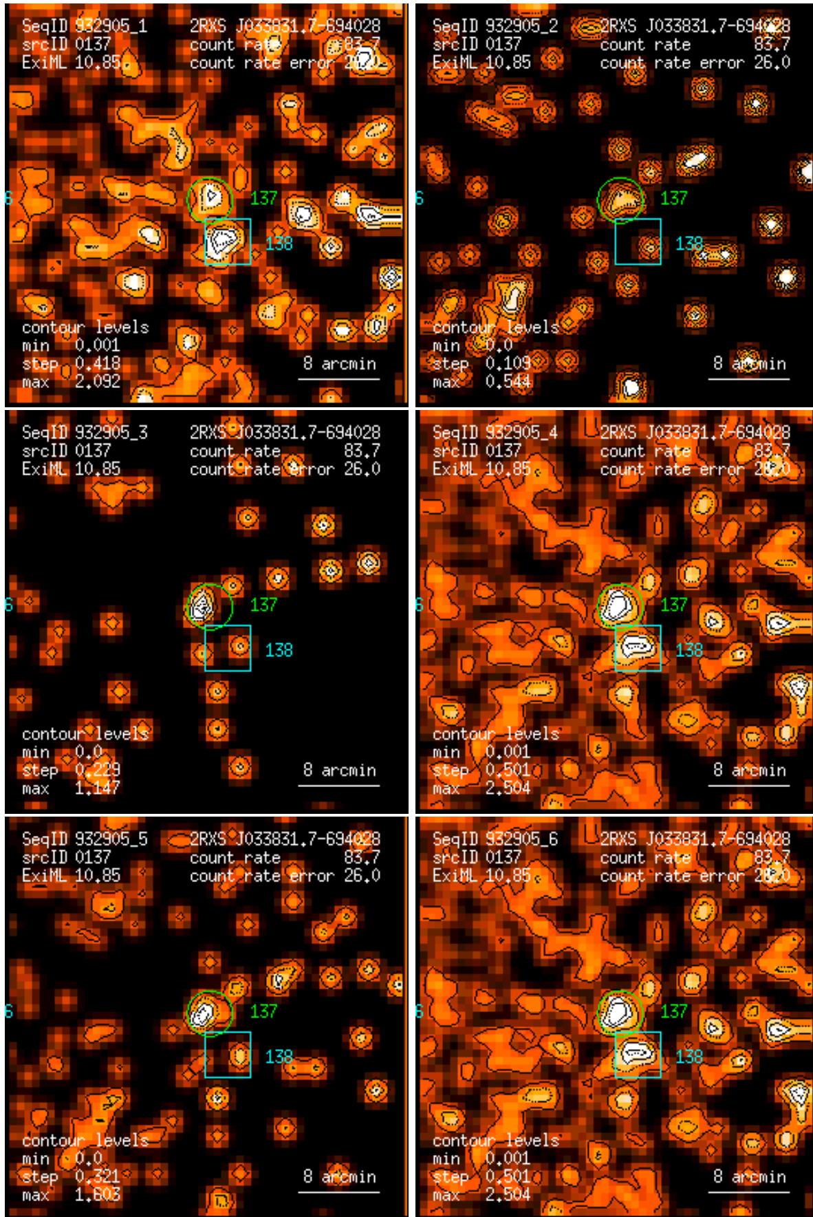
Figure 137: RASS 932905: detection 0137: band rate images, Gaussian filter: (1) PSPC channels 11 – 41, (2) 52 – 90, (3) 91 – 201, (4) 11 – 235, (5) 52 – 201, (6) 11 – 201. Broad band rates in counts/ks. Band rate contour levels in counts/ks/arcmin 2 .
