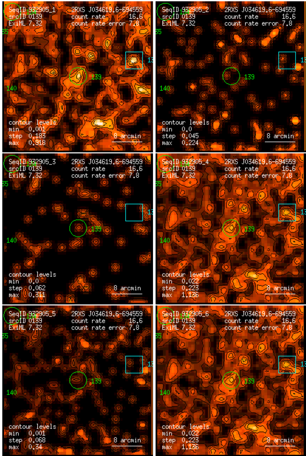
Figure 139: RASS 932905: detection 0139: band rate images, Gaussian filter: (1) PSPC channels 11 – 41, (2) 52 – 90, (3) 91 – 201, (4) 11 – 235, (5) 52 – 201, (6) 11 – 201. Broad band rates in counts/ks. Band rate contour levels in counts/ks/arcmin 2 .
