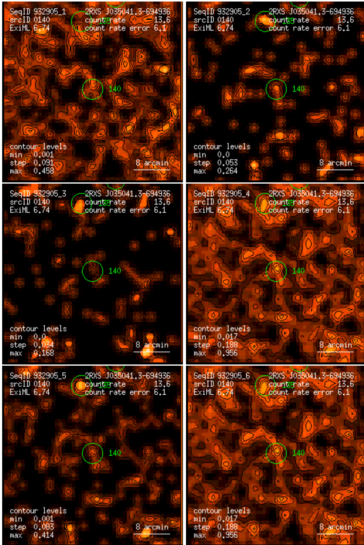
Figure 140: RASS 932905: detection 0140: band rate images, Gaussian filter: (1) PSPC channels 11 – 41, (2) 52 – 90, (3) 91 – 201, (4) 11 – 235, (5) 52 – 201, (6) 11 – 201. Broad band rates in counts/ks. Band rate contour levels in counts/ks/arcmin 2 .
