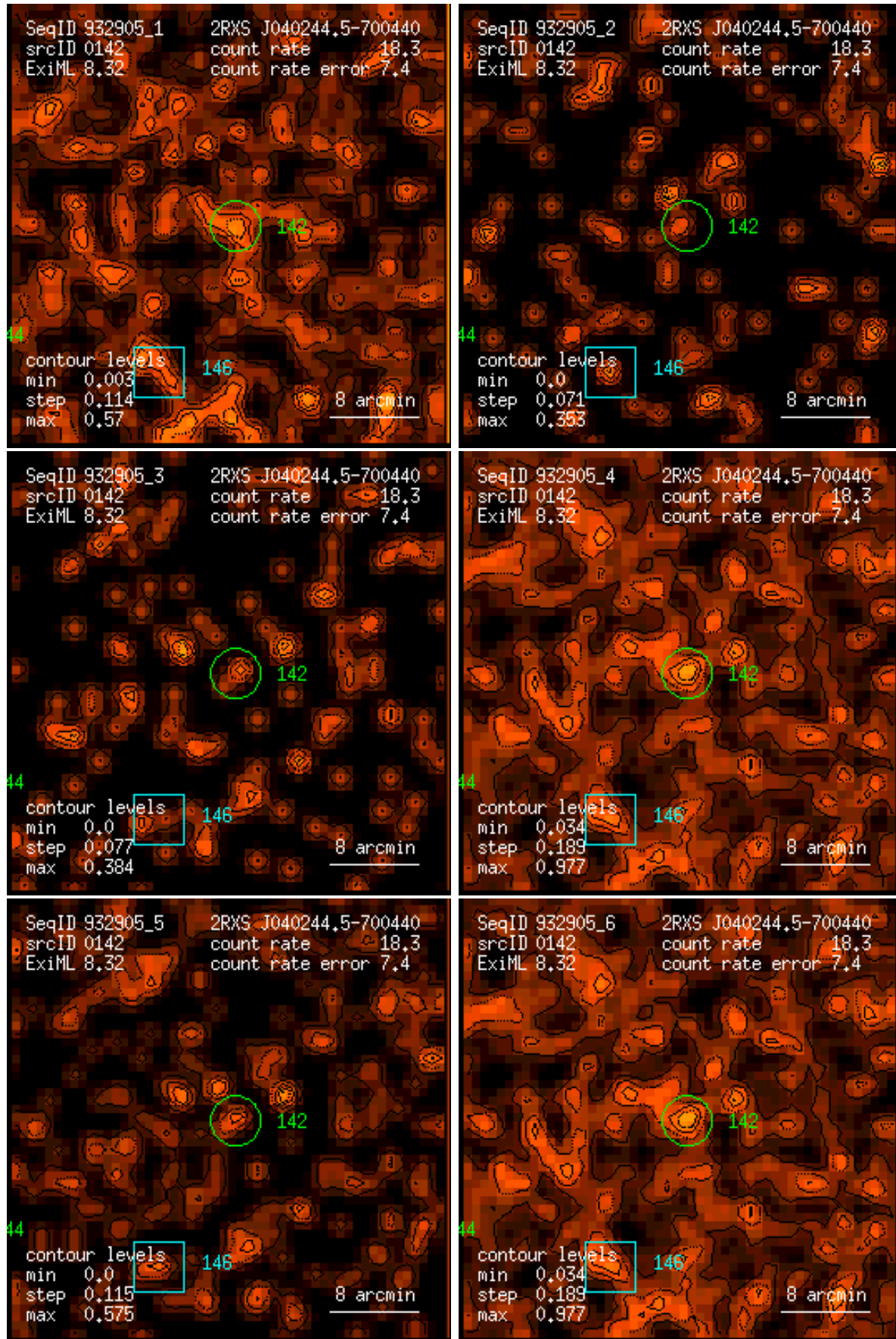
Figure 142: RASS 932905: detection 0142: band rate images, Gaussian filter: (1) PSPC channels 11 – 41, (2) 52 – 90, (3) 91 – 201, (4) 11 – 235, (5) 52 – 201, (6) 11 – 201. Broad band rates in counts/ks. Band rate contour levels in counts/ks/arcmin 2 .
