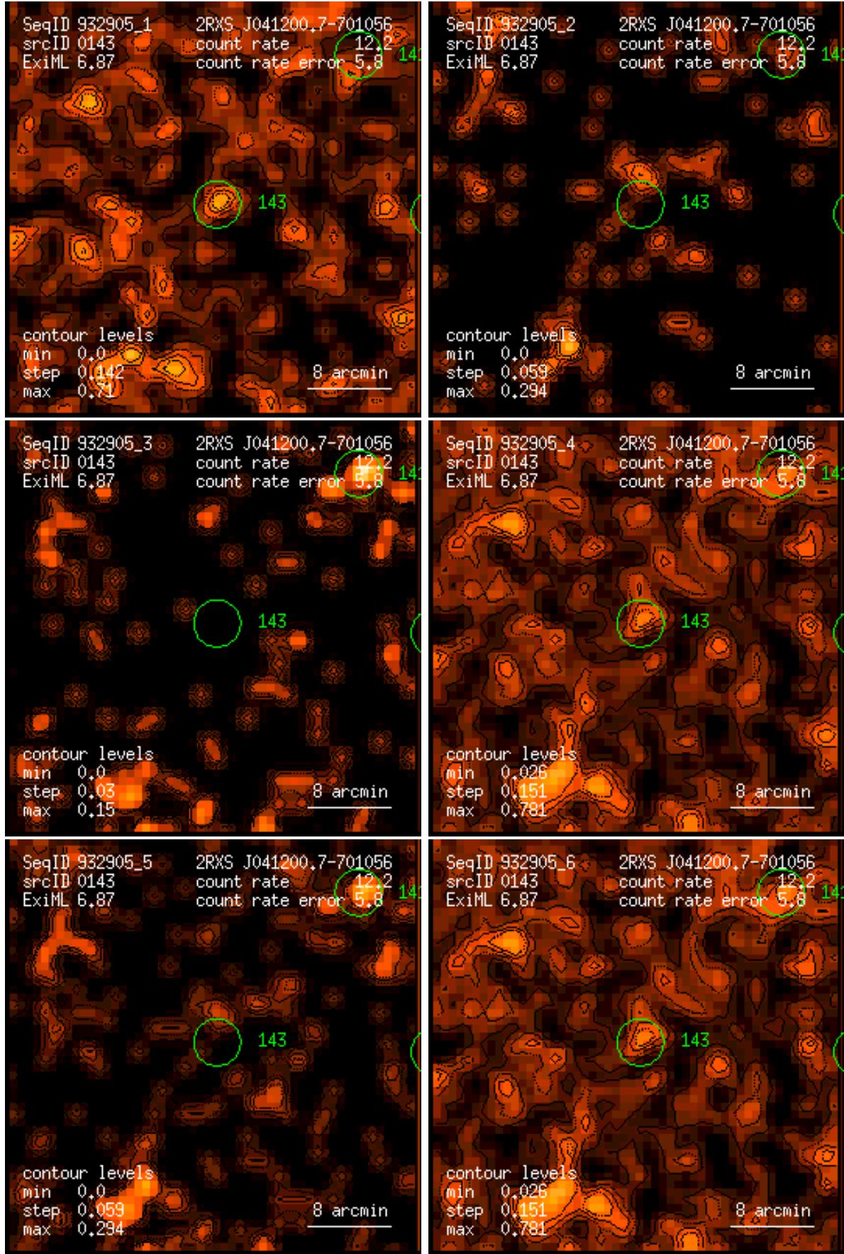
Figure 143: RASS 932905: detection 0143: band rate images, Gaussian filter: (1) PSPC channels 11 – 41, (2) 52 – 90, (3) 91 – 201, (4) 11 – 235, (5) 52 – 201, (6) 11 – 201. Broad band rates in counts/ks. Band rate contour levels in counts/ks/arcmin 2 .
