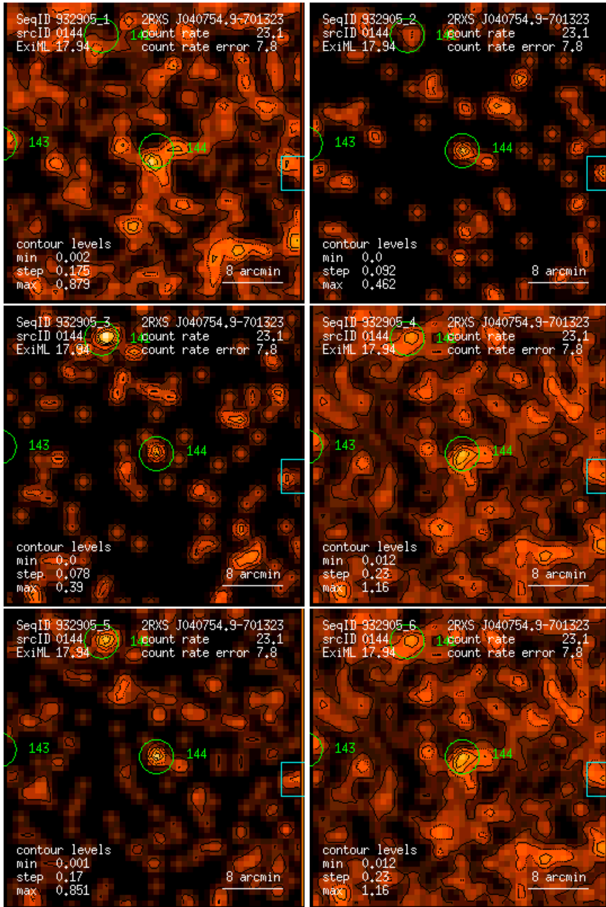
Figure 144: RASS 932905: detection 0144: band rate images, Gaussian filter: (1) PSPC channels 11 – 41, (2) 52 – 90, (3) 91 – 201, (4) 11 – 235, (5) 52 – 201, (6) 11 – 201. Broad band rates in counts/ks. Band rate contour levels in counts/ks/arcmin 2 .
