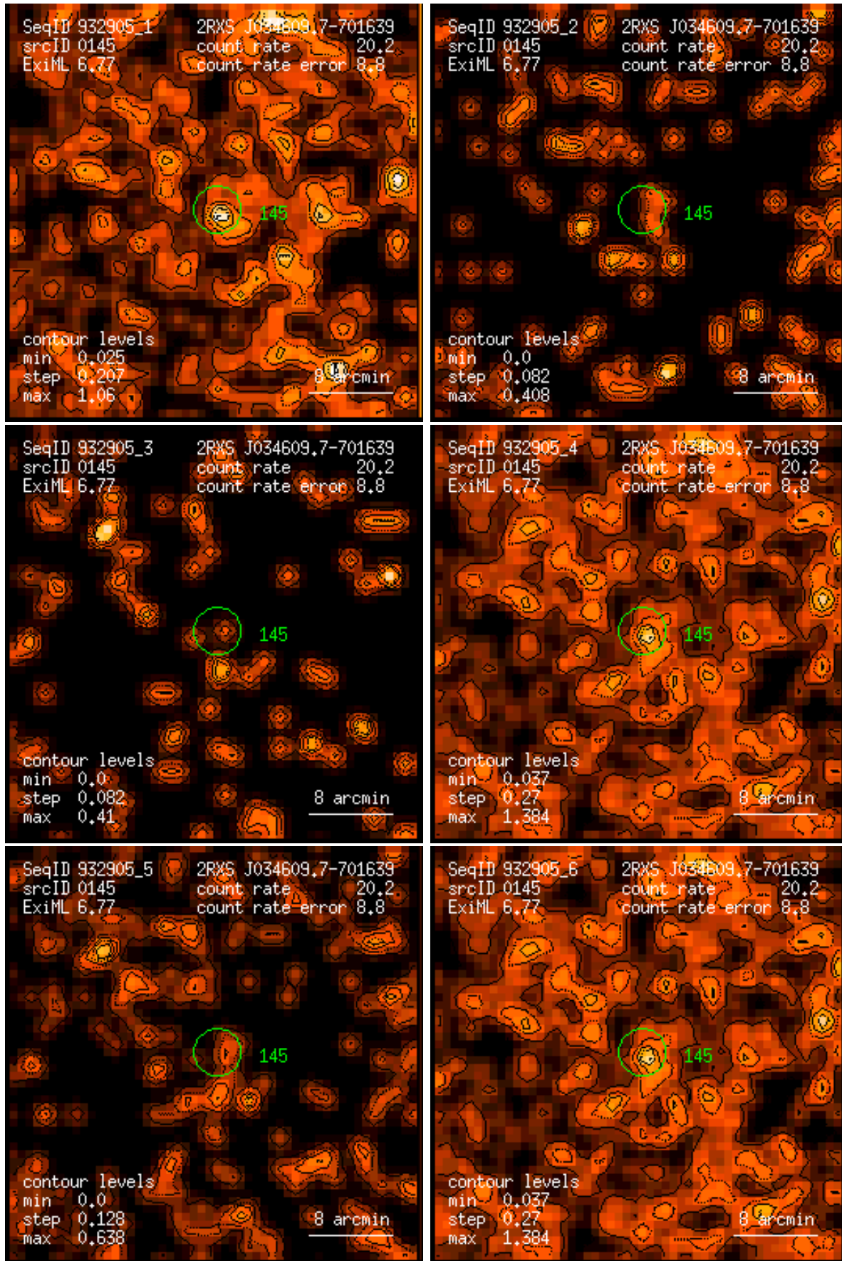
Figure 145: RASS 932905: detection 0145: band rate images, Gaussian filter: (1) PSPC channels 11 – 41, (2) 52 – 90, (3) 91 – 201, (4) 11 – 235, (5) 52 – 201, (6) 11 – 201. Broad band rates in counts/ks. Band rate contour levels in counts/ks/arcmin 2 .
