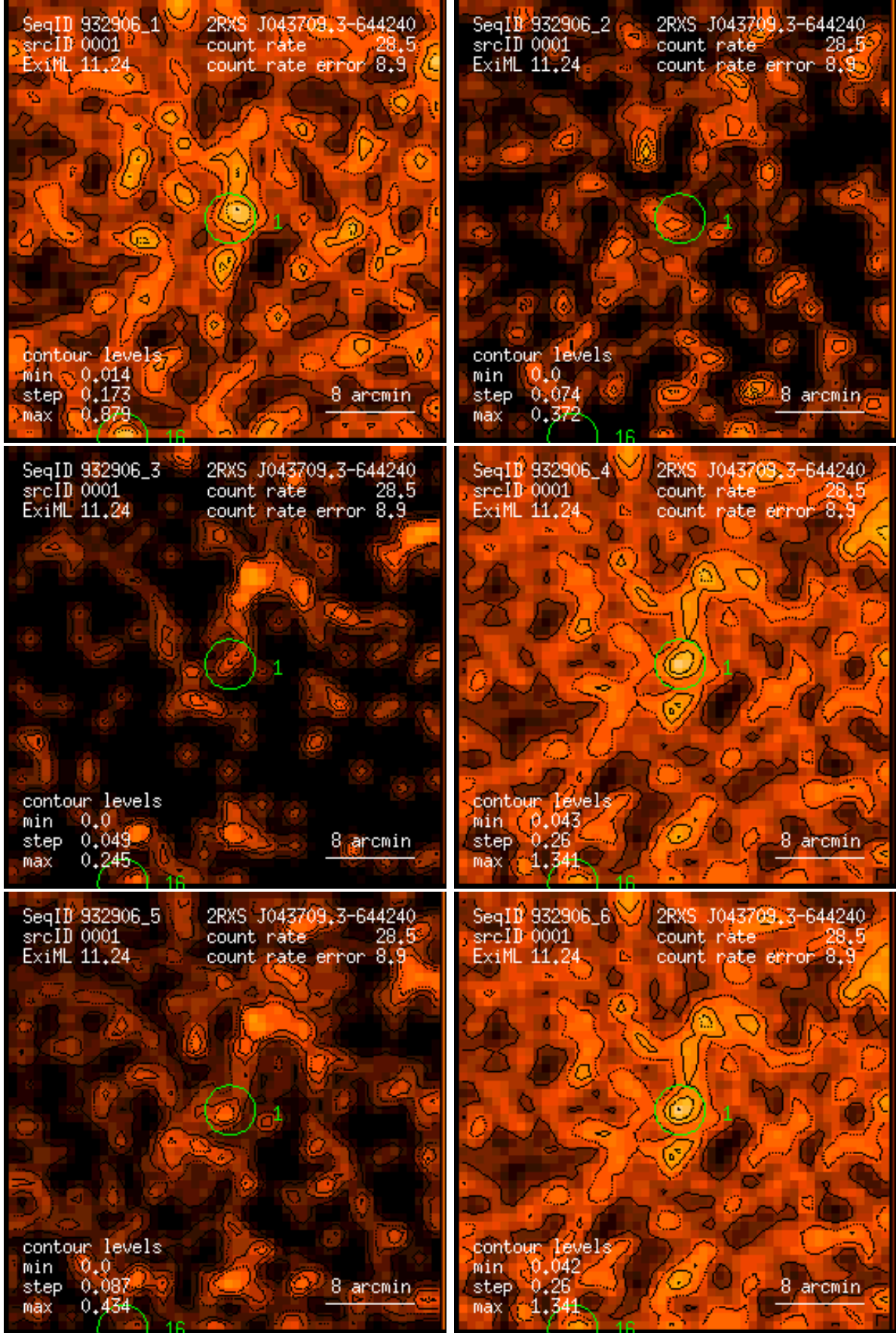
Figure 1: RASS 932906: detection 0001: band rate images, Gaussian filter: (1) PSPC channels 11 – 41, (2) 52 – 90, (3) 91 – 201, (4) 11 – 235, (5) 52 – 201, (6) 11 – 201. Broad band rates in counts/ks. Band rate contour levels in counts/ks/arcmin 2 .
