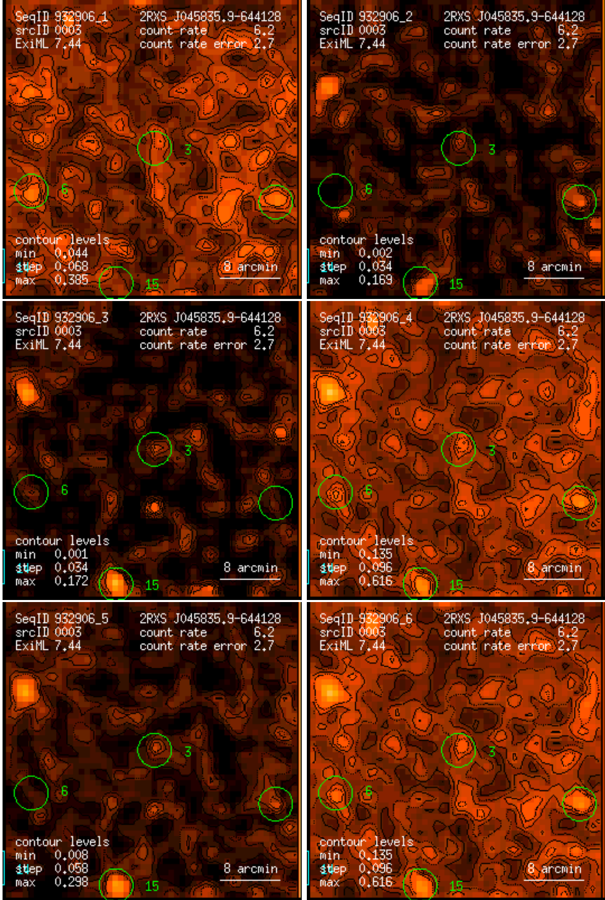
Figure 3: RASS 932906: detection 0003: band rate images, Gaussian filter: (1) PSPC channels 11 – 41, (2) 52 – 90, (3) 91 – 201, (4) 11 – 235, (5) 52 – 201, (6) 11 – 201. Broad band rates in counts/ks. Band rate contour levels in counts/ks/arcmin 2 .
