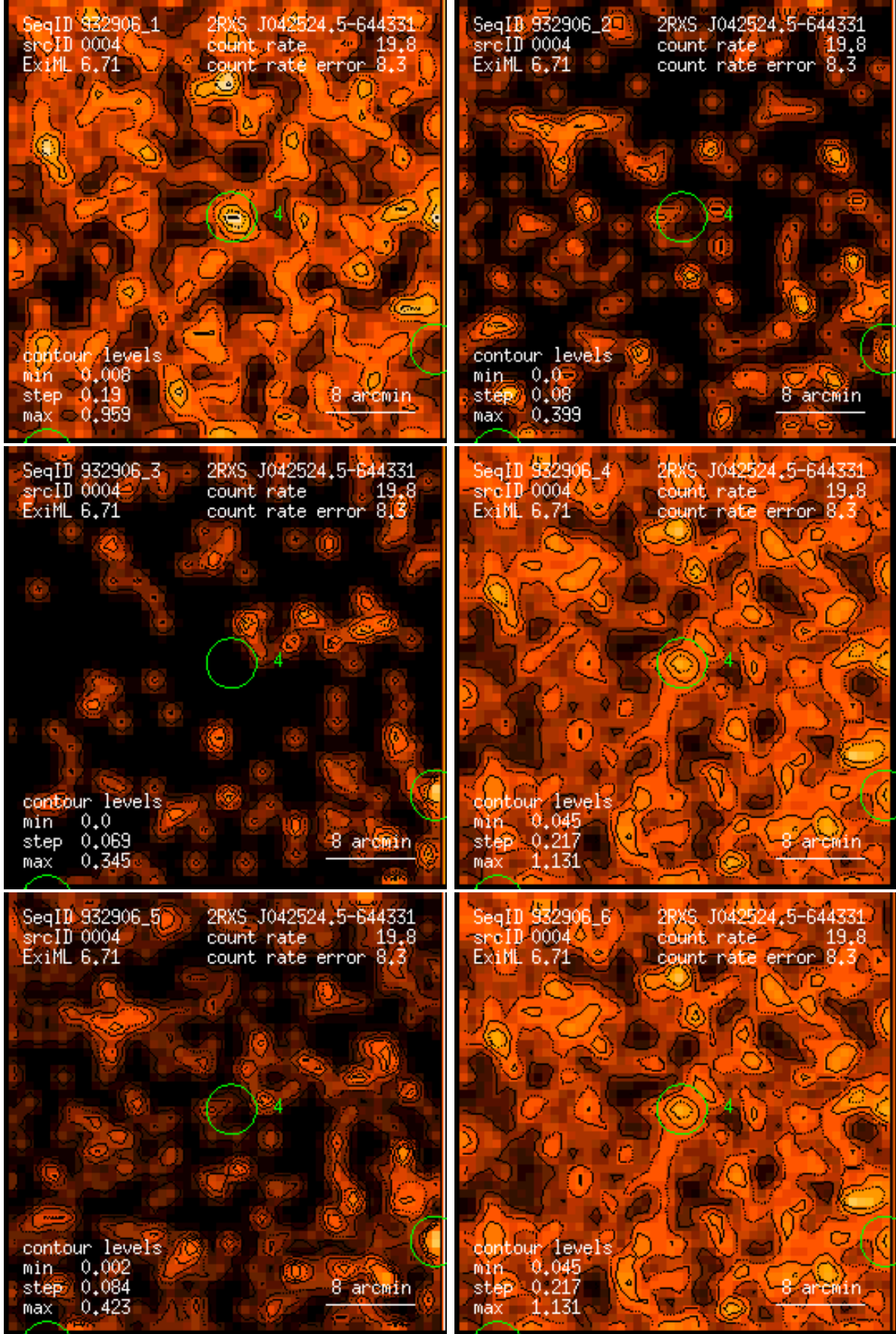
Figure 4: RASS 932906: detection 0004: band rate images, Gaussian filter: (1) PSPC channels 11 – 41, (2) 52 – 90, (3) 91 – 201, (4) 11 – 235, (5) 52 – 201, (6) 11 – 201. Broad band rates in counts/ks. Band rate contour levels in counts/ks/arcmin 2 .
