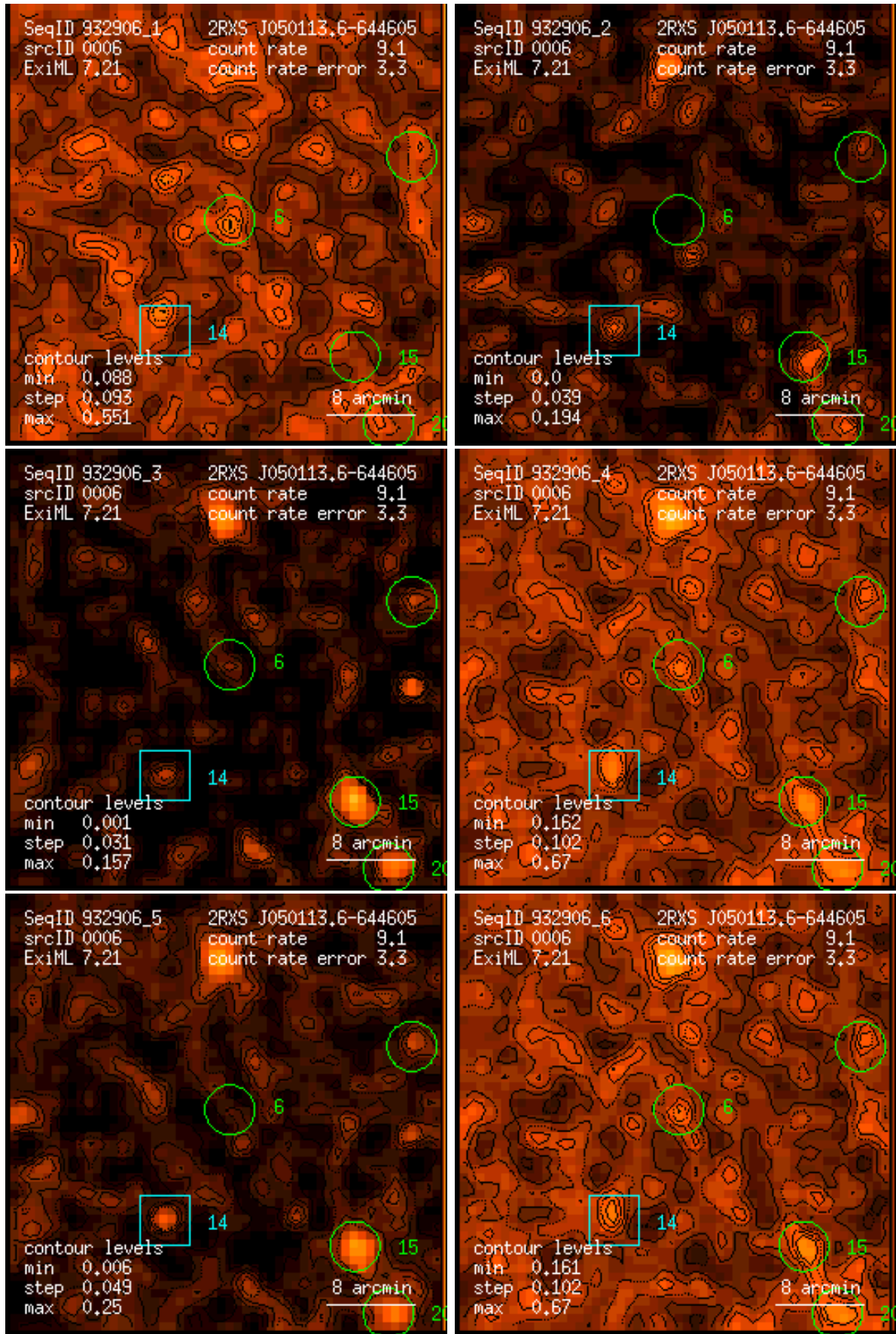
Figure 6: RASS 932906: detection 0006: band rate images, Gaussian filter: (1) PSPC channels 11 – 41, (2) 52 – 90, (3) 91 – 201, (4) 11 – 235, (5) 52 – 201, (6) 11 – 201. Broad band rates in counts/ks. Band rate contour levels in counts/ks/arcmin 2 .
