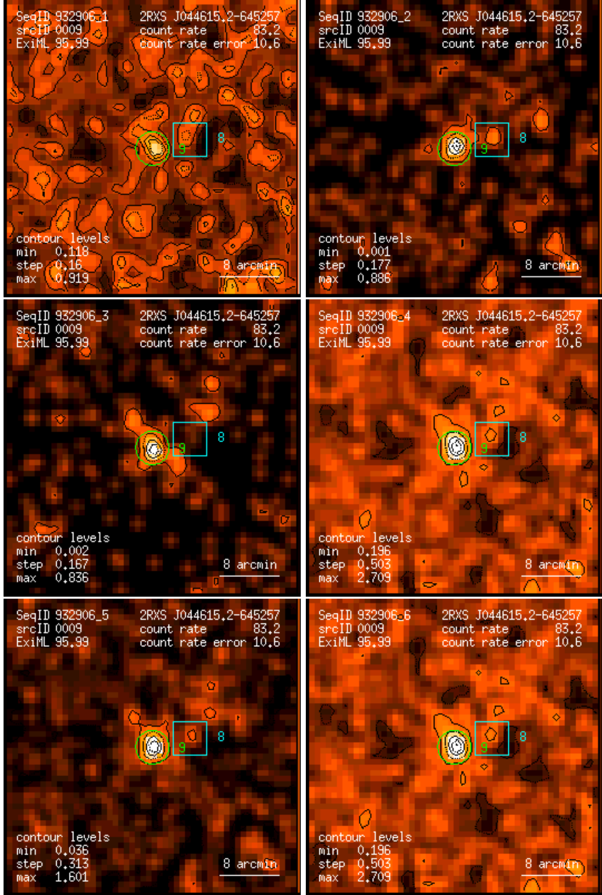
Figure 9: RASS 932906: detection 0009: band rate images, Gaussian filter: (1) PSPC channels 11 – 41, (2) 52 – 90, (3) 91 – 201, (4) 11 – 235, (5) 52 – 201, (6) 11 – 201. Broad band rates in counts/ks. Band rate contour levels in counts/ks/arcmin 2 .
