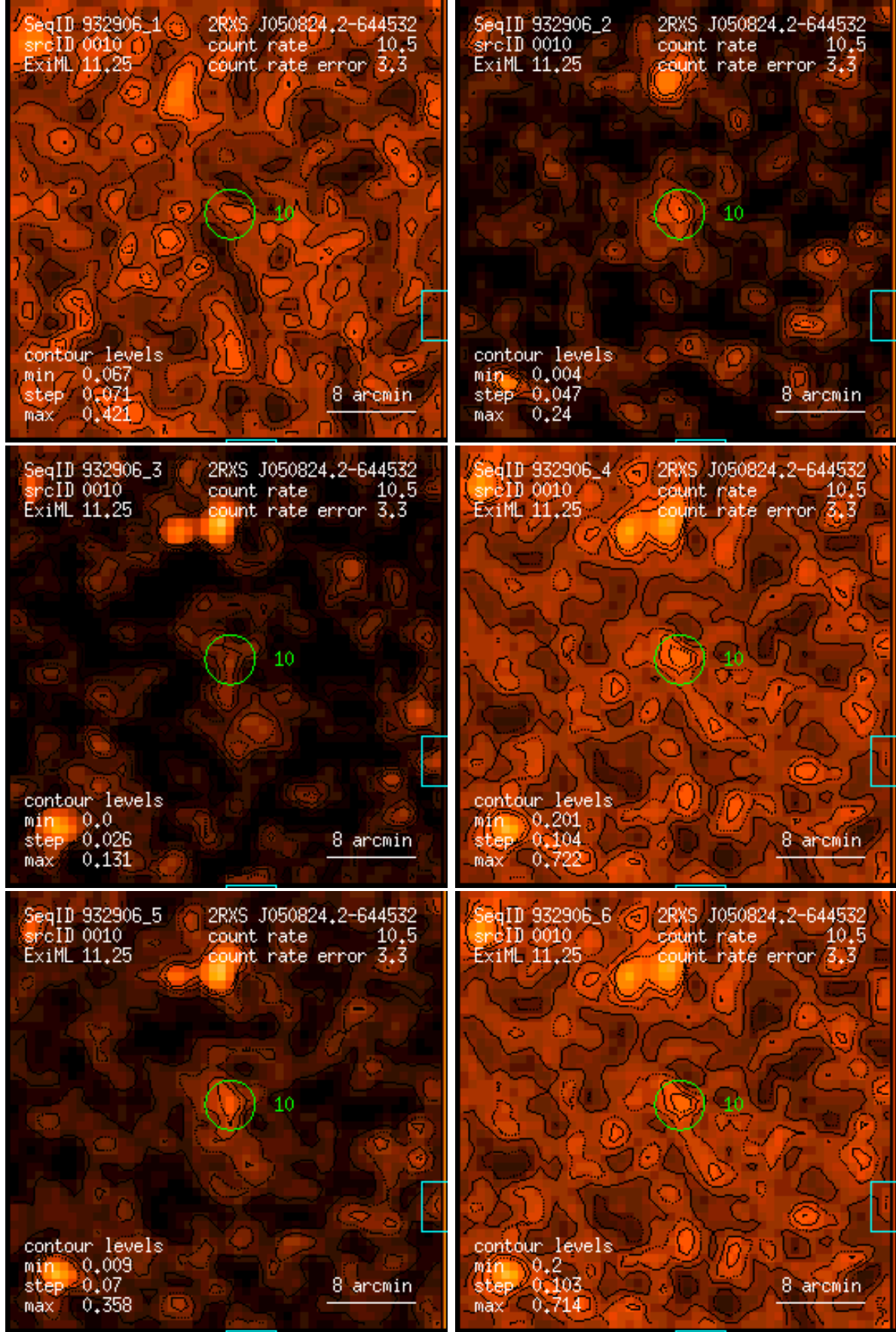
Figure 10: RASS 932906: detection 0010: band rate images, Gaussian filter: (1) PSPC channels 11 – 41, (2) 52 – 90, (3) 91 – 201, (4) 11 – 235, (5) 52 – 201, (6) 11 – 201. Broad band rates in counts/ks. Band rate contour levels in counts/ks/arcmin 2 .
