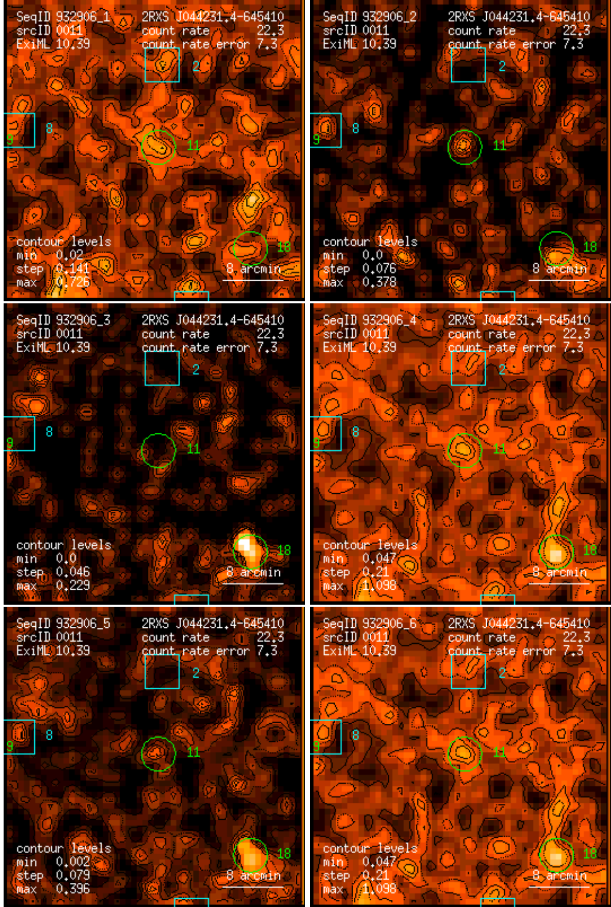
Figure 11: RASS 932906: detection 0011: band rate images, Gaussian filter: (1) PSPC channels 11 – 41, (2) 52 – 90, (3) 91 – 201, (4) 11 – 235, (5) 52 – 201, (6) 11 – 201. Broad band rates in counts/ks. Band rate contour levels in counts/ks/arcmin 2 .
