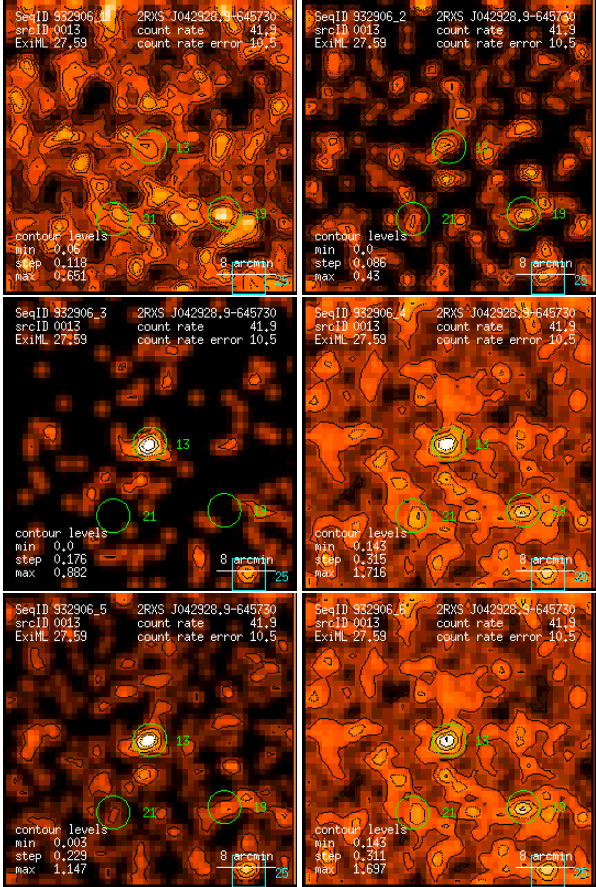
Figure 13: RASS 932906: detection 0013: band rate images, Gaussian filter: (1) PSPC channels 11 – 41, (2) 52 – 90, (3) 91 – 201, (4) 11 – 235, (5) 52 – 201, (6) 11 – 201. Broad band rates in counts/ks. Band rate contour levels in counts/ks/arcmin 2 .
