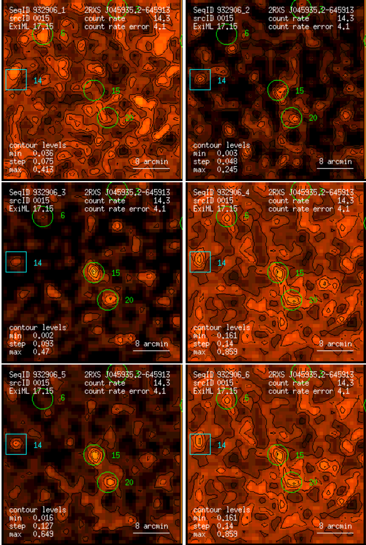
Figure 15: RASS 932906: detection 0015: band rate images, Gaussian filter: (1) PSPC channels 11 – 41, (2) 52 – 90, (3) 91 – 201, (4) 11 – 235, (5) 52 – 201, (6) 11 – 201. Broad band rates in counts/ks. Band rate contour levels in counts/ks/arcmin 2 .
