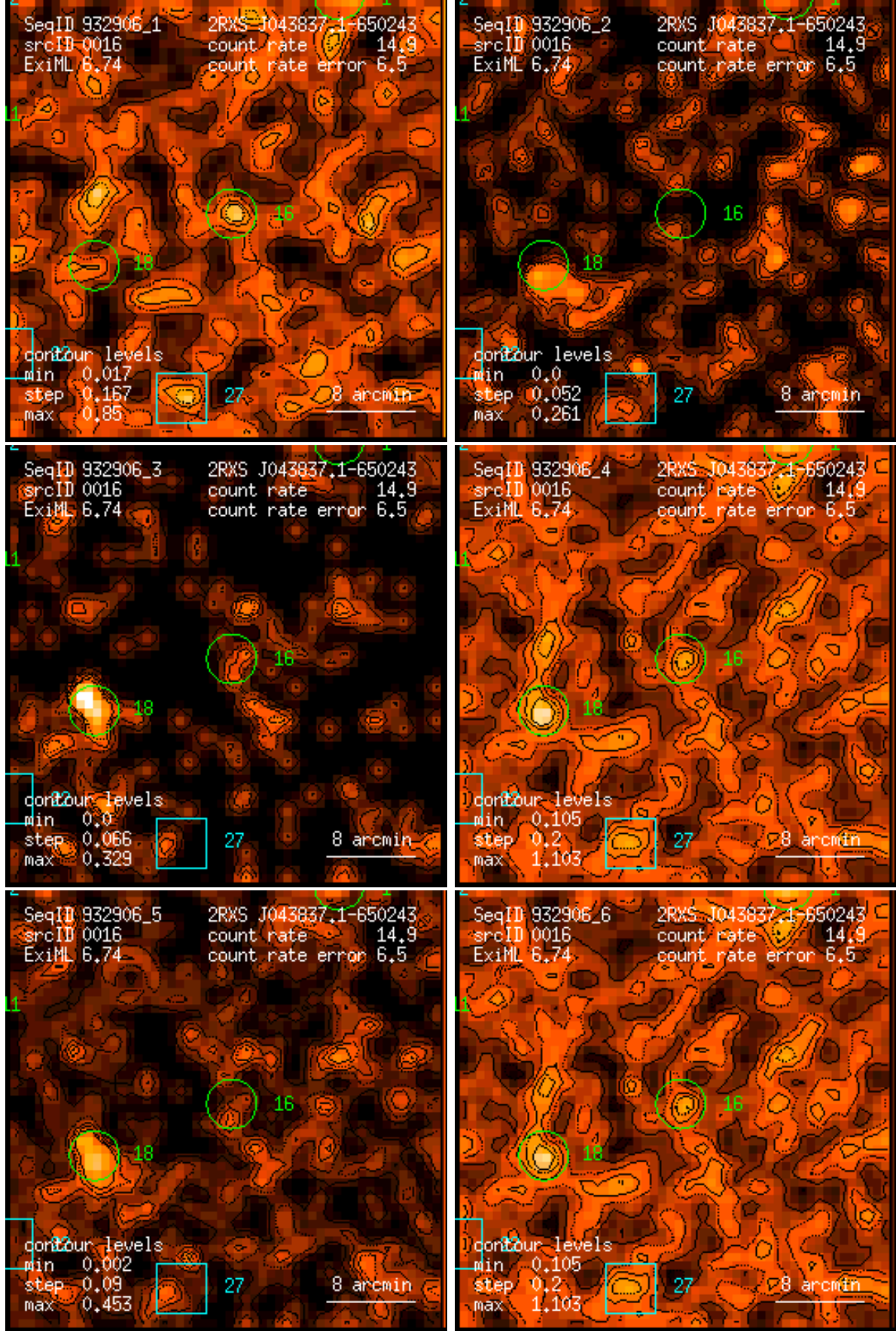
Figure 16: RASS 932906: detection 0016: band rate images, Gaussian filter: (1) PSPC channels 11 – 41, (2) 52 – 90, (3) 91 – 201, (4) 11 – 235, (5) 52 – 201, (6) 11 – 201. Broad band rates in counts/ks. Band rate contour levels in counts/ks/arcmin 2 .
