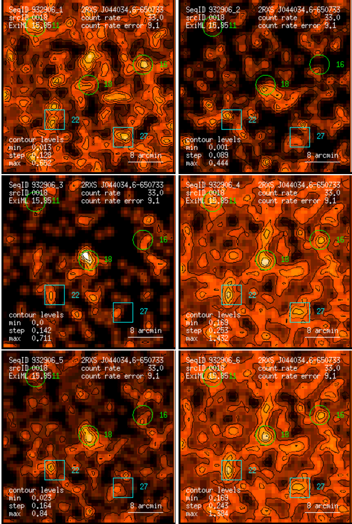
Figure 18: RASS 932906: detection 0018: band rate images, Gaussian filter: (1) PSPC channels 11 – 41, (2) 52 – 90, (3) 91 – 201, (4) 11 – 235, (5) 52 – 201, (6) 11 – 201. Broad band rates in counts/ks. Band rate contour levels in counts/ks/arcmin 2 .
