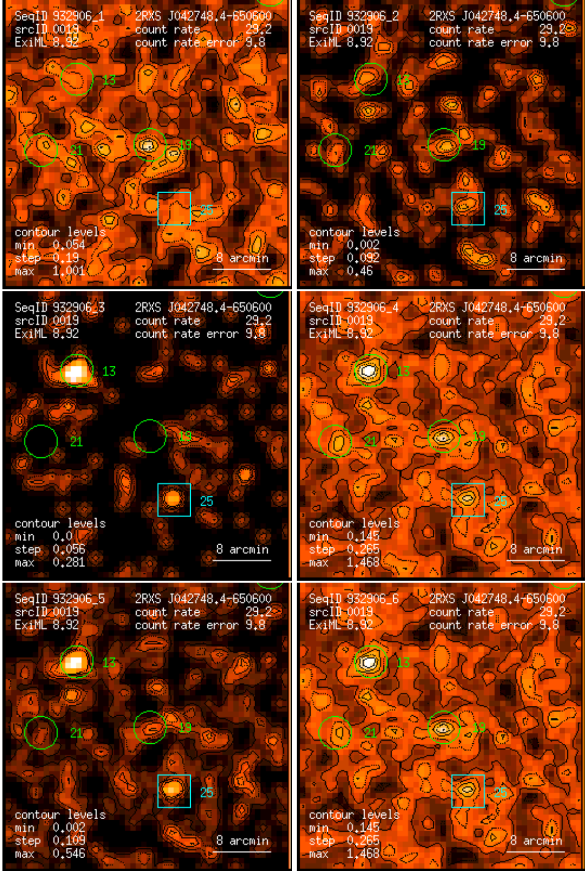
Figure 19: RASS 932906: detection 0019: band rate images, Gaussian filter: (1) PSPC channels 11 – 41, (2) 52 – 90, (3) 91 – 201, (4) 11 – 235, (5) 52 – 201, (6) 11 – 201. Broad band rates in counts/ks. Band rate contour levels in counts/ks/arcmin 2 .
