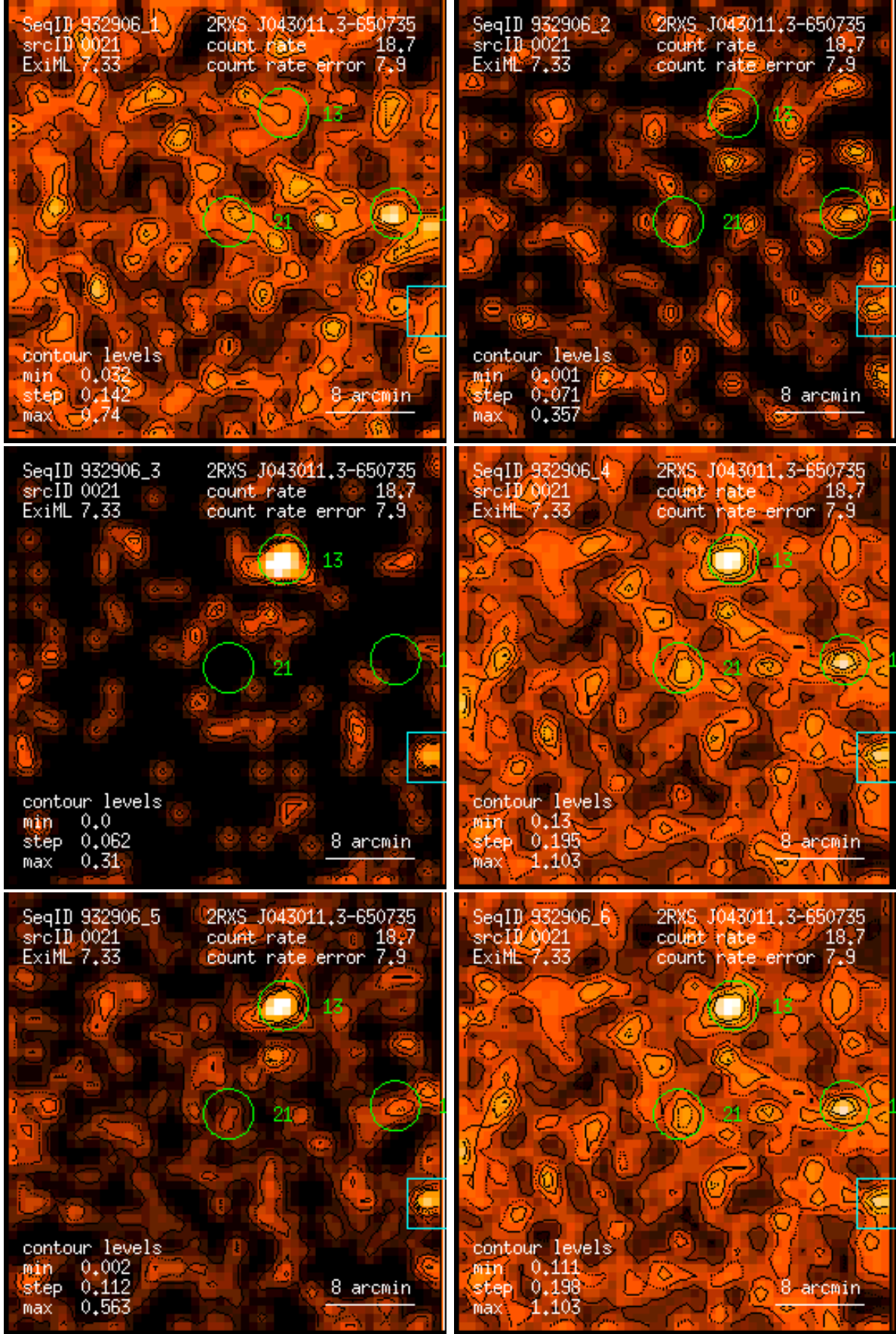
Figure 21: RASS 932906: detection 0021: band rate images, Gaussian filter: (1) PSPC channels 11 – 41, (2) 52 – 90, (3) 91 – 201, (4) 11 – 235, (5) 52 – 201, (6) 11 – 201. Broad band rates in counts/ks. Band rate contour levels in counts/ks/arcmin 2 .
