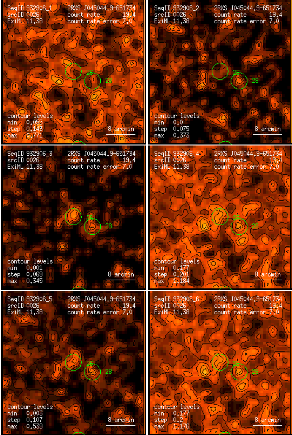
Figure 26: RASS 932906: detection 0026: band rate images, Gaussian filter: (1) PSPC channels 11 – 41, (2) 52 – 90, (3) 91 – 201, (4) 11 – 235, (5) 52 – 201, (6) 11 – 201. Broad band rates in counts/ks. Band rate contour levels in counts/ks/arcmin 2 .
