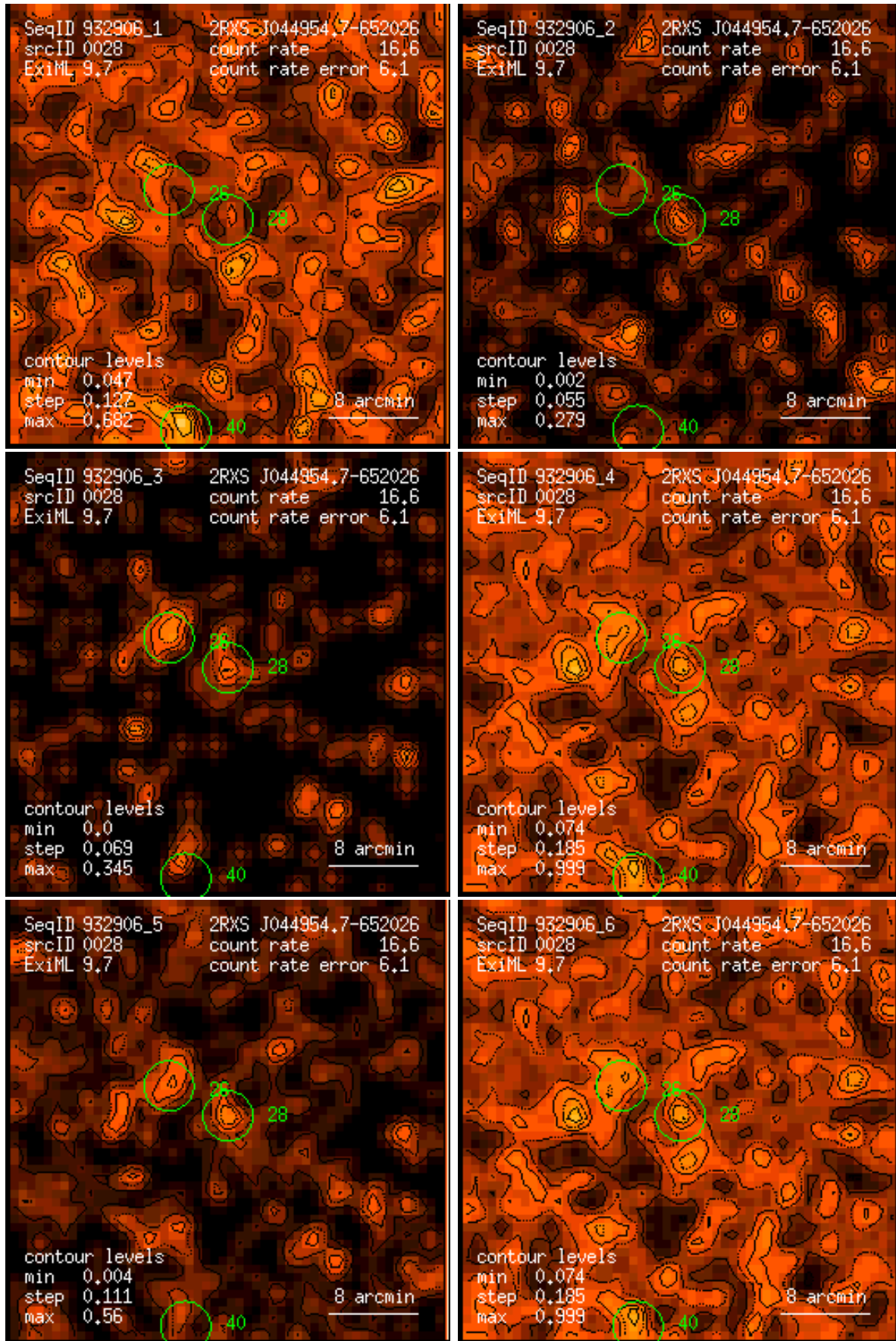
Figure 28: RASS 932906: detection 0028: band rate images, Gaussian filter: (1) PSPC channels 11 – 41, (2) 52 – 90, (3) 91 – 201, (4) 11 – 235, (5) 52 – 201, (6) 11 – 201. Broad band rates in counts/ks. Band rate contour levels in counts/ks/arcmin 2 .
