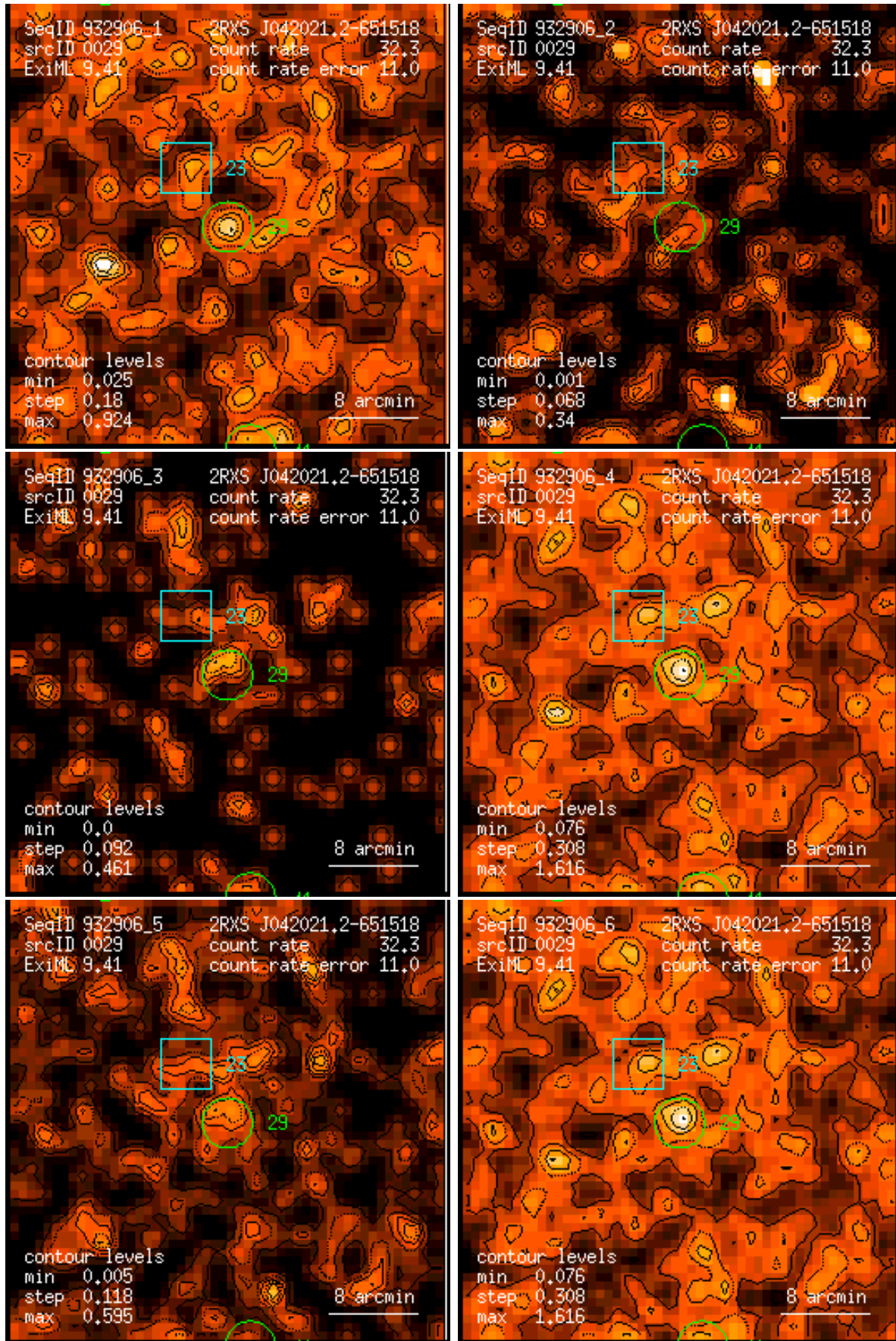
Figure 29: RASS 932906: detection 0029: band rate images, Gaussian filter: (1) PSPC channels 11 – 41, (2) 52 – 90, (3) 91 – 201, (4) 11 – 235, (5) 52 – 201, (6) 11 – 201. Broad band rates in counts/ks. Band rate contour levels in counts/ks/arcmin 2 .
