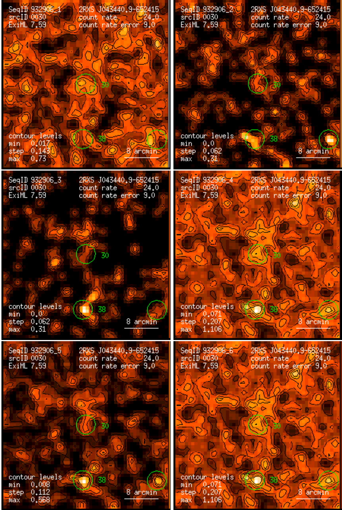
Figure 30: RASS 932906: detection 0030: band rate images, Gaussian filter: (1) PSPC channels 11 – 41, (2) 52 – 90, (3) 91 – 201, (4) 11 – 235, (5) 52 – 201, (6) 11 – 201. Broad band rates in counts/ks. Band rate contour levels in counts/ks/arcmin 2 .
