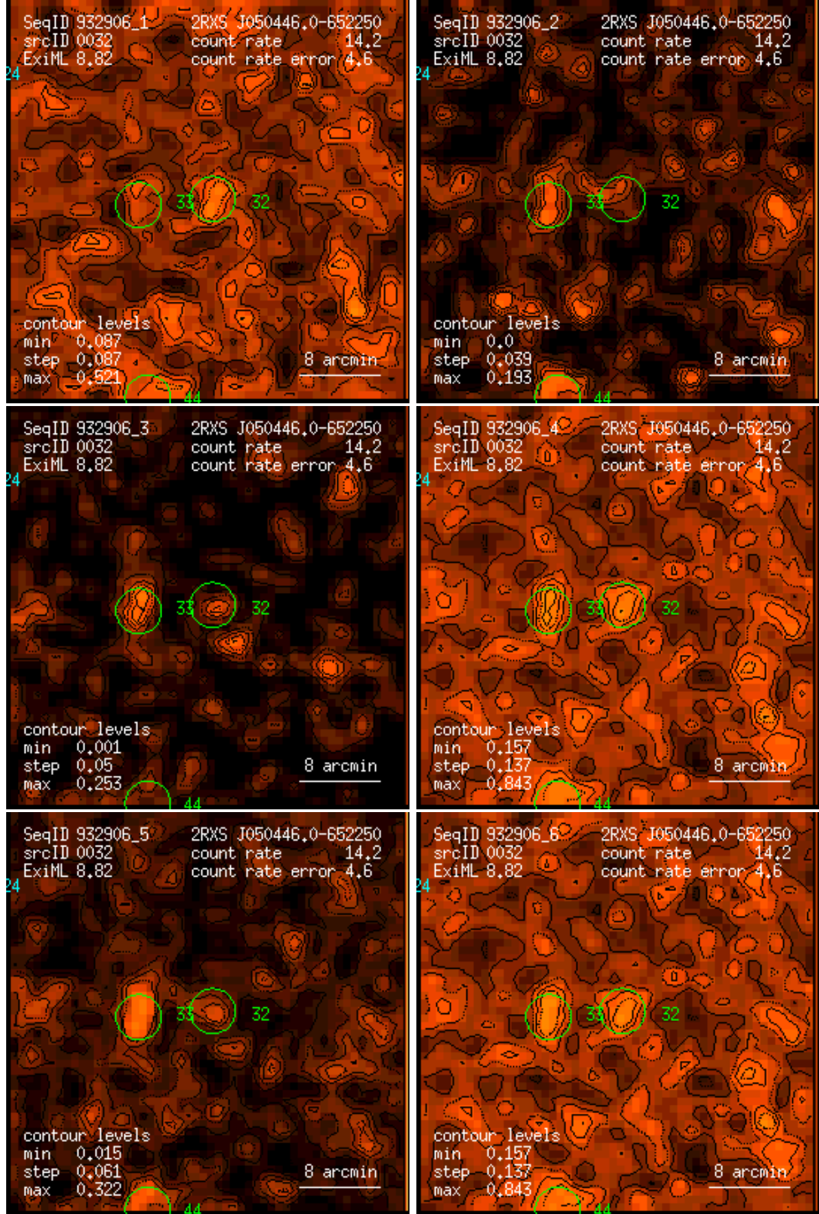
Figure 32: RASS 932906: detection 0032: band rate images, Gaussian filter: (1) PSPC channels 11 – 41, (2) 52 – 90, (3) 91 – 201, (4) 11 – 235, (5) 52 – 201, (6) 11 – 201. Broad band rates in counts/ks. Band rate contour levels in counts/ks/arcmin 2 .
