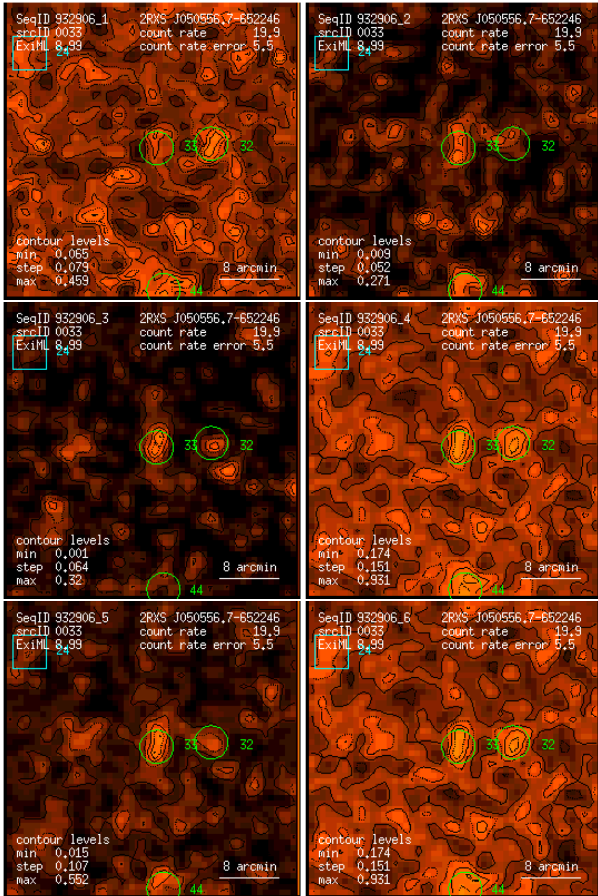
Figure 33: RASS 932906: detection 0033: band rate images, Gaussian filter: (1) PSPC channels 11 – 41, (2) 52 – 90, (3) 91 – 201, (4) 11 – 235, (5) 52 – 201, (6) 11 – 201. Broad band rates in counts/ks. Band rate contour levels in counts/ks/arcmin 2 .
