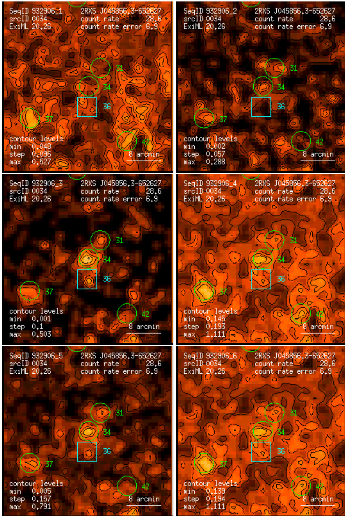
Figure 34: RASS 932906: detection 0034: band rate images, Gaussian filter: (1) PSPC channels 11 – 41, (2) 52 – 90, (3) 91 – 201, (4) 11 – 235, (5) 52 – 201, (6) 11 – 201. Broad band rates in counts/ks. Band rate contour levels in counts/ks/arcmin 2 .
