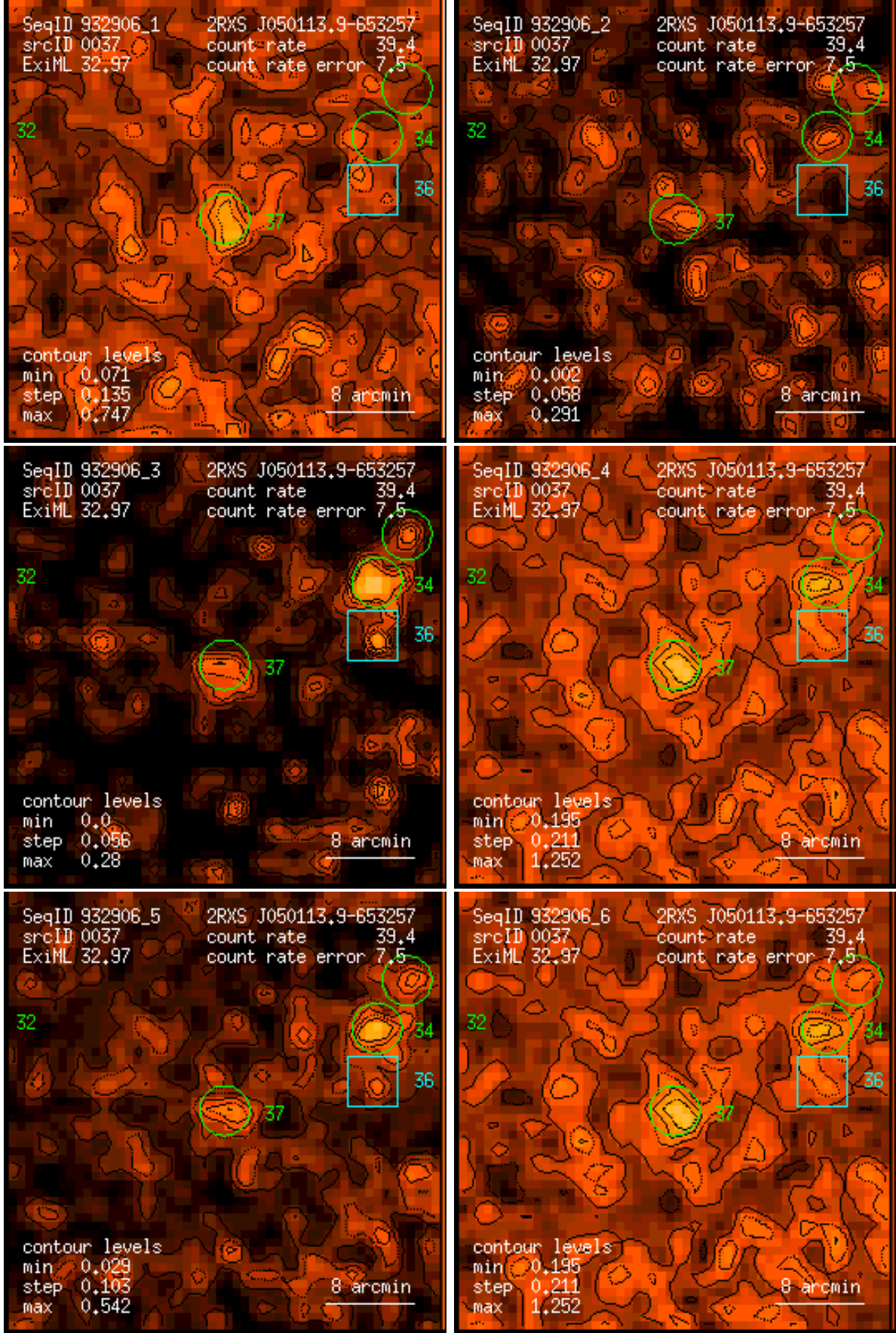
Figure 37: RASS 932906: detection 0037: band rate images, Gaussian filter: (1) PSPC channels 11 – 41, (2) 52 – 90, (3) 91 – 201, (4) 11 – 235, (5) 52 – 201, (6) 11 – 201. Broad band rates in counts/ks. Band rate contour levels in counts/ks/arcmin 2 .
