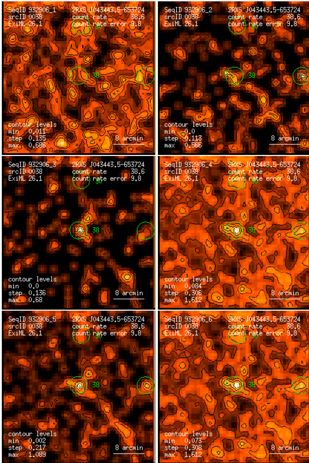
Figure 38: RASS 932906: detection 0038: band rate images, Gaussian filter: (1) PSPC channels 11 – 41, (2) 52 – 90, (3) 91 – 201, (4) 11 – 235, (5) 52 – 201, (6) 11 – 201. Broad band rates in counts/ks. Band rate contour levels in counts/ks/arcmin 2 .
