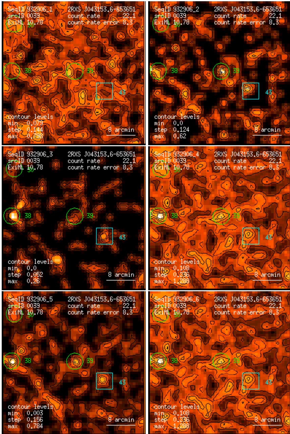
Figure 39: RASS 932906: detection 0039: band rate images, Gaussian filter: (1) PSPC channels 11 – 41, (2) 52 – 90, (3) 91 – 201, (4) 11 – 235, (5) 52 – 201, (6) 11 – 201. Broad band rates in counts/ks. Band rate contour levels in counts/ks/arcmin 2 .
