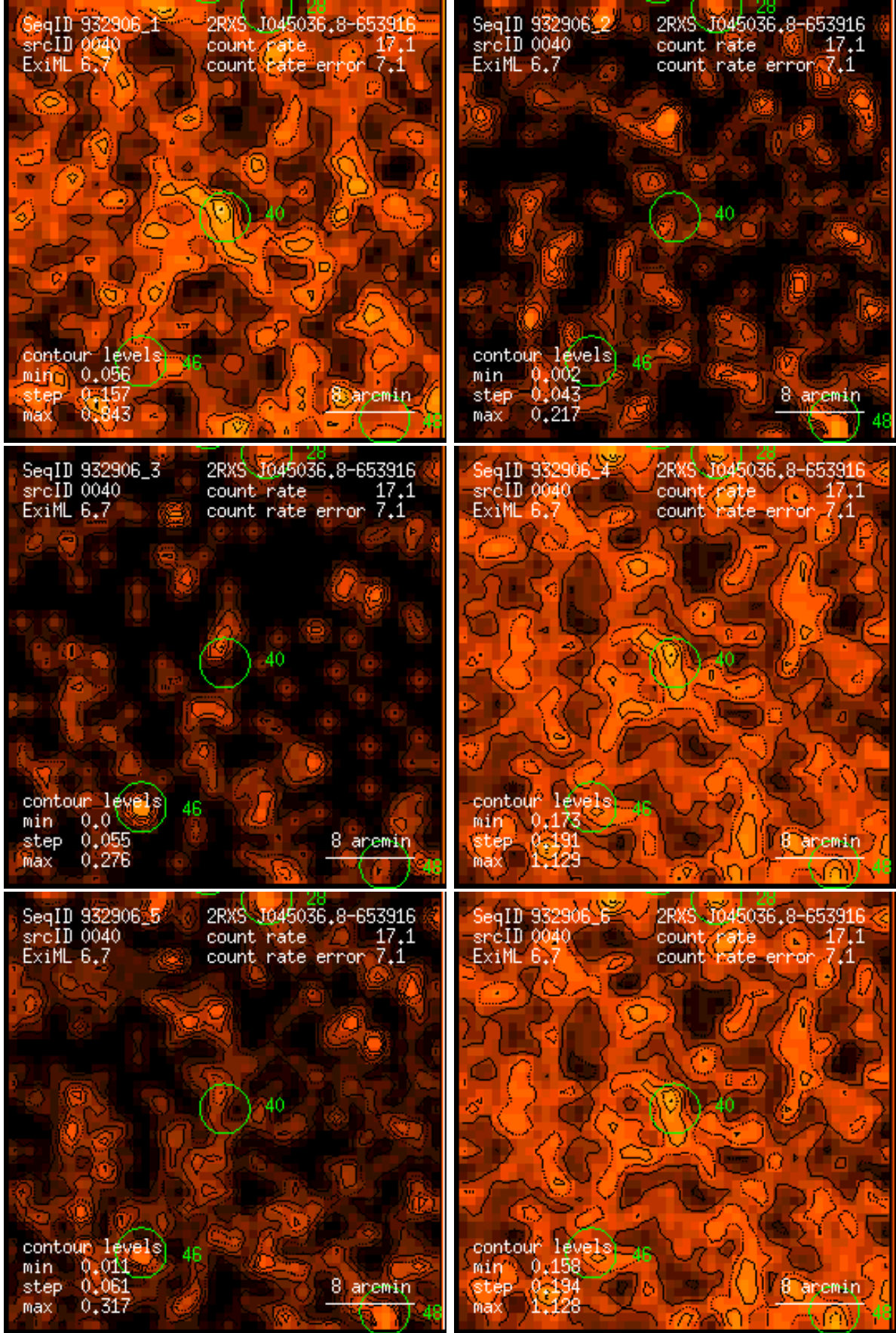
Figure 40: RASS 932906: detection 0040: band rate images, Gaussian filter: (1) PSPC channels 11 – 41, (2) 52 – 90, (3) 91 – 201, (4) 11 – 235, (5) 52 – 201, (6) 11 – 201. Broad band rates in counts/ks. Band rate contour levels in counts/ks/arcmin 2 .
