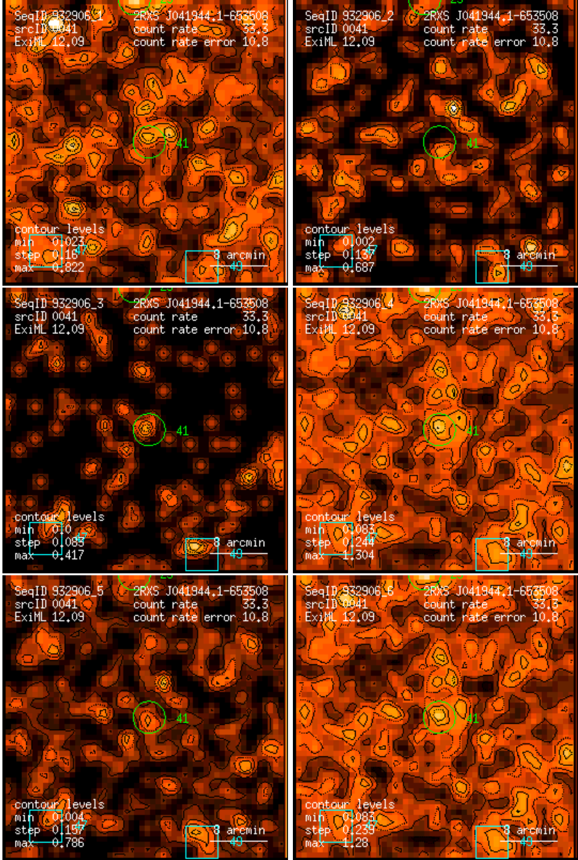
Figure 41: RASS 932906: detection 0041: band rate images, Gaussian filter: (1) PSPC channels 11 – 41, (2) 52 – 90, (3) 91 – 201, (4) 11 – 235, (5) 52 – 201, (6) 11 – 201. Broad band rates in counts/ks. Band rate contour levels in counts/ks/arcmin 2 .
