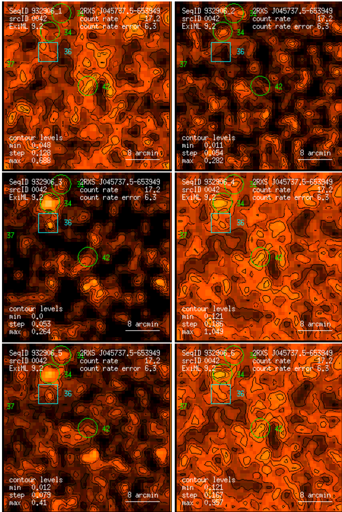
Figure 42: RASS 932906: detection 0042: band rate images, Gaussian filter: (1) PSPC channels 11 – 41, (2) 52 – 90, (3) 91 – 201, (4) 11 – 235, (5) 52 – 201, (6) 11 – 201. Broad band rates in counts/ks. Band rate contour levels in counts/ks/arcmin 2 .
