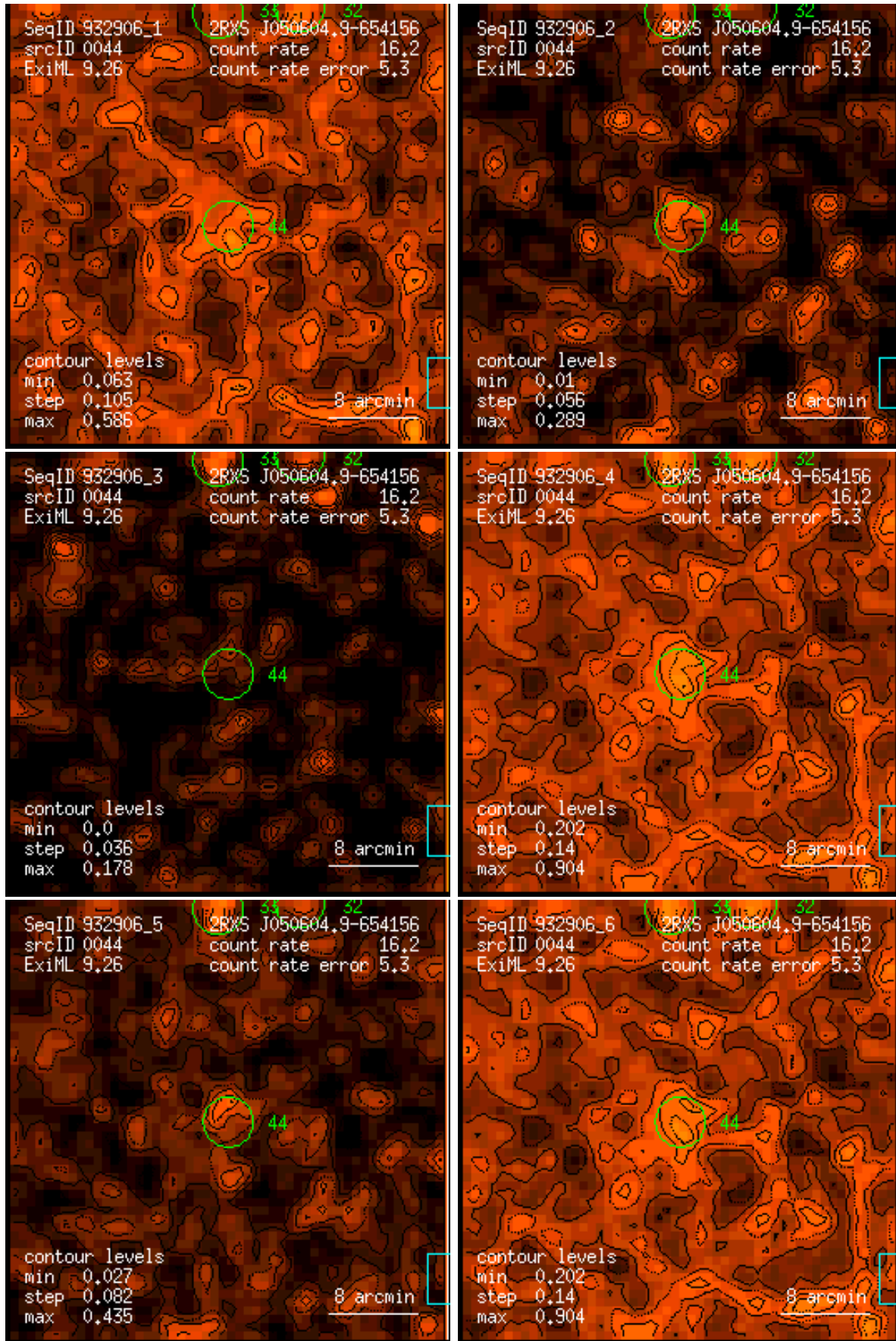
Figure 44: RASS 932906: detection 0044: band rate images, Gaussian filter: (1) PSPC channels 11 – 41, (2) 52 – 90, (3) 91 – 201, (4) 11 – 235, (5) 52 – 201, (6) 11 – 201. Broad band rates in counts/ks. Band rate contour levels in counts/ks/arcmin 2 .
