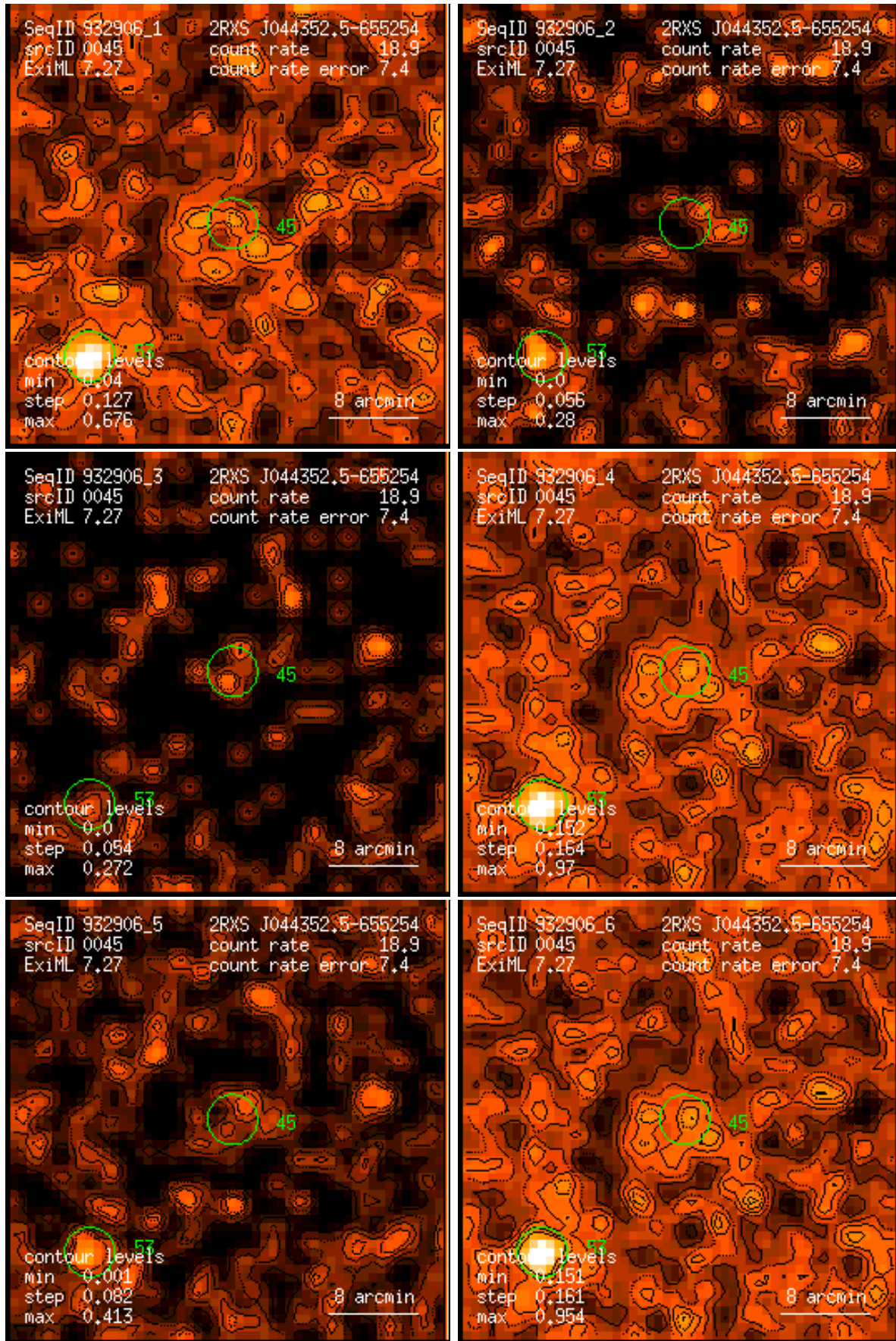
Figure 45: RASS 932906: detection 0045: band rate images, Gaussian filter: (1) PSPC channels 11 – 41, (2) 52 – 90, (3) 91 – 201, (4) 11 – 235, (5) 52 – 201, (6) 11 – 201. Broad band rates in counts/ks. Band rate contour levels in counts/ks/arcmin 2 .
