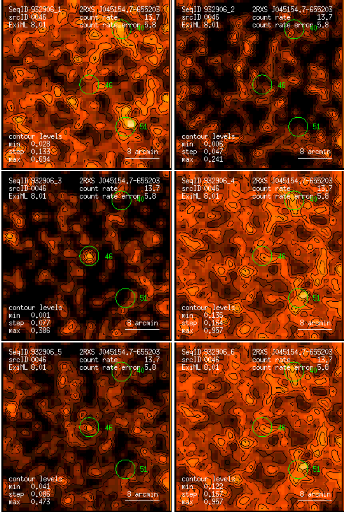
Figure 46: RASS 932906: detection 0046: band rate images, Gaussian filter: (1) PSPC channels 11 – 41, (2) 52 – 90, (3) 91 – 201, (4) 11 – 235, (5) 52 – 201, (6) 11 – 201. Broad band rates in counts/ks. Band rate contour levels in counts/ks/arcmin 2 .
