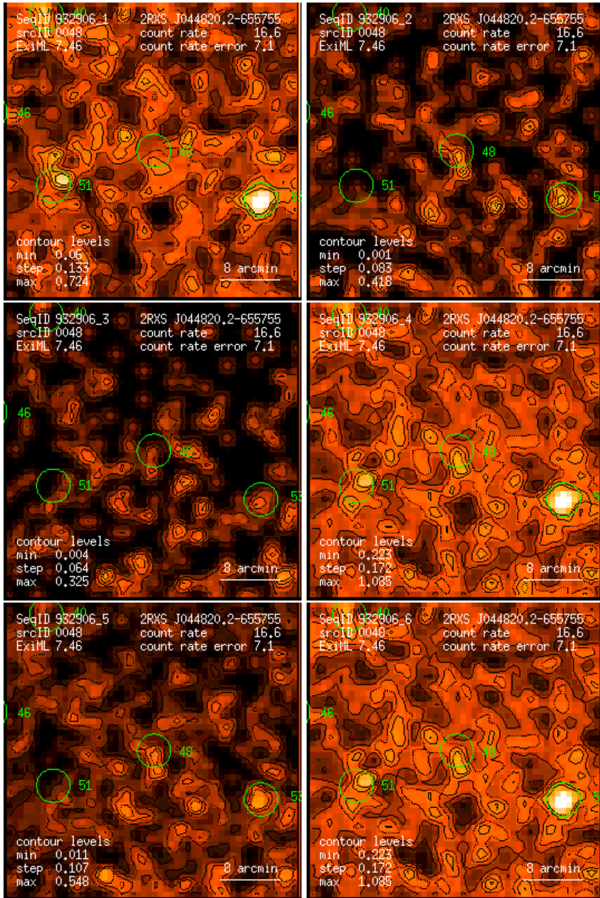
Figure 48: RASS 932906: detection 0048: band rate images, Gaussian filter: (1) PSPC channels 11 – 41, (2) 52 – 90, (3) 91 – 201, (4) 11 – 235, (5) 52 – 201, (6) 11 – 201. Broad band rates in counts/ks. Band rate contour levels in counts/ks/arcmin 2 .
